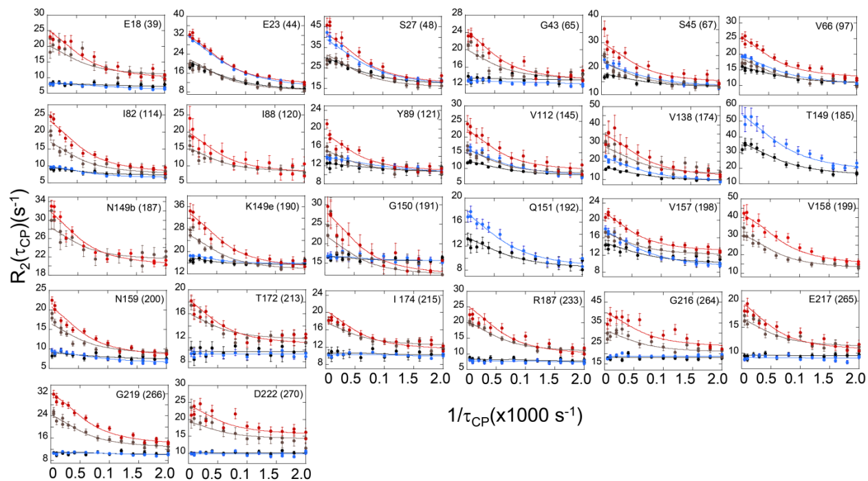
Supplementary Figure 1. Relaxation dispersion curves for apo-thrombin (800 MHz in red, 600 MHz in brown) and PPACK-thrombin (800 MHz in blue, 600 MHz in black). Curves are global fits from GLOVE.
