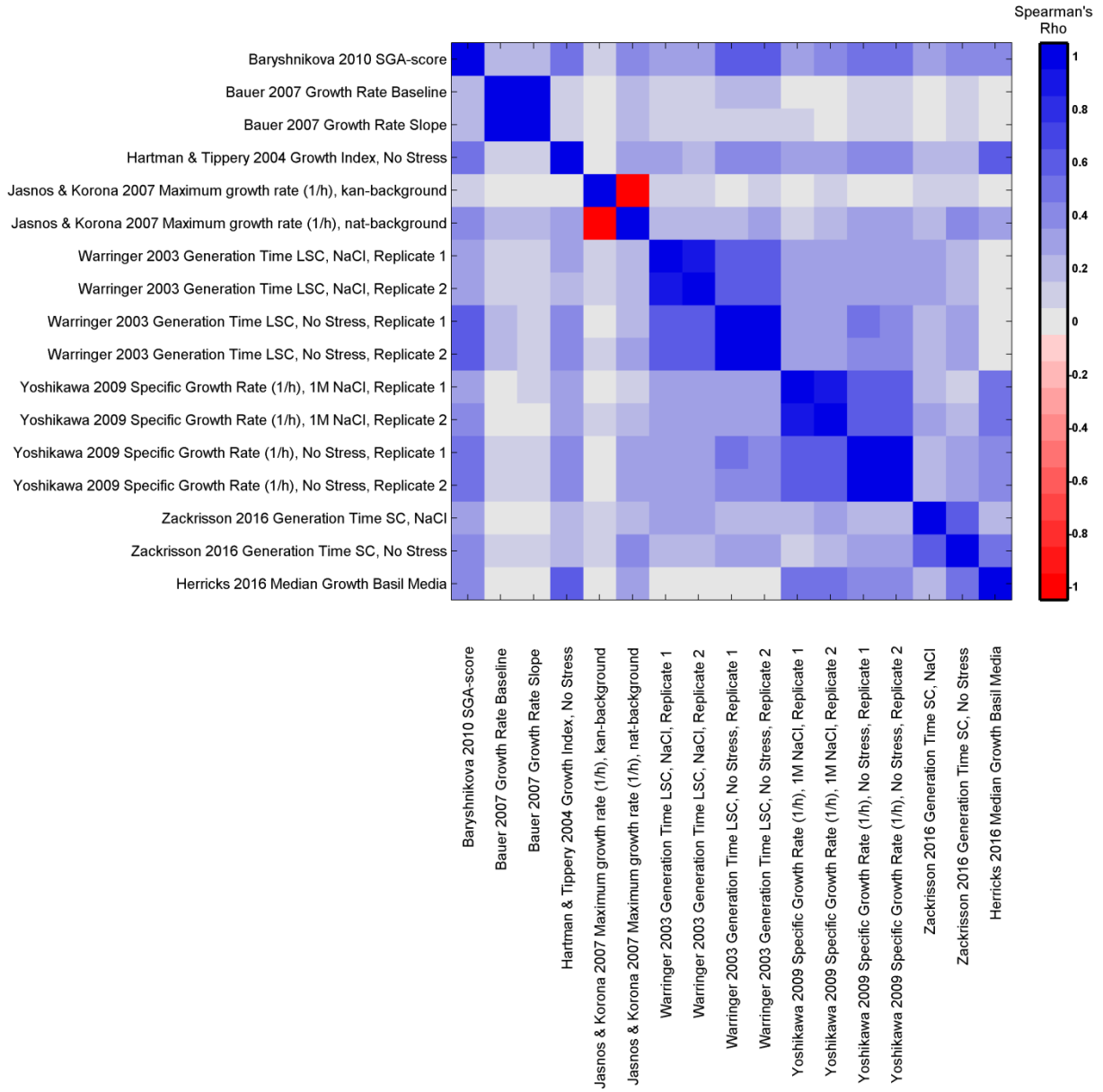
Figure S1: Spearman's Rho rank correlation coefficient with other previously published studies. This figure was generated with data originally published elsewhere and generously shared for by M. Zackrisson and A. Blomberg (Zackrisson et al., 2016). The ODELAY data set is relatively small but shows modest correlations with other datasets. Overall correlation
