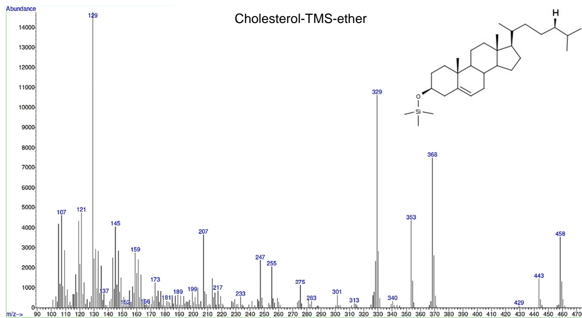
S8 Fig. Mass spectrum and structural formula of cholesterol trimethylsilyl ether.
