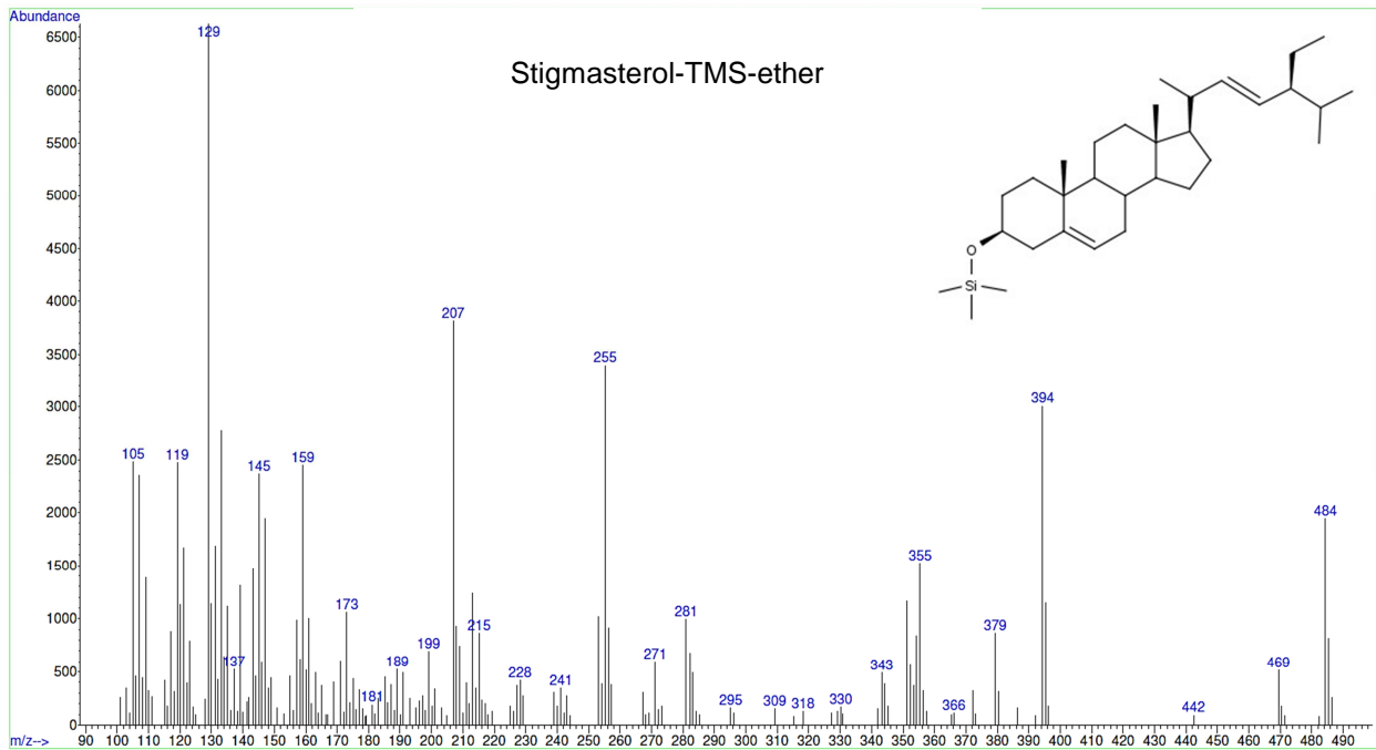
S10 Fig. Mass spectrum and structural formula of stigmasterol trimethylsilyl ether.
