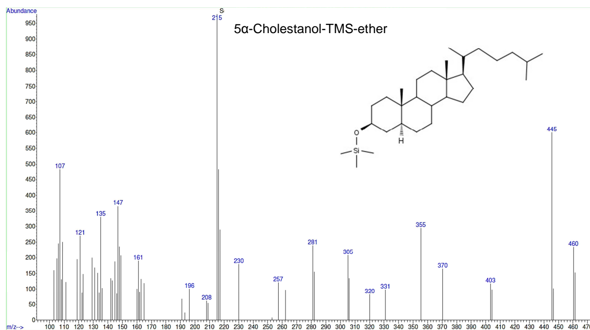
S11 Fig. Mass spectrum and structural formula of 5α-cholestanol trimethylsilyl ether.
