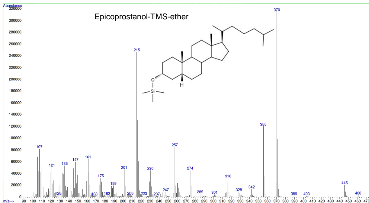
S13 Fig. Mass spectrum and structural formula of epicoprostanol trimethylsilyl ether.
