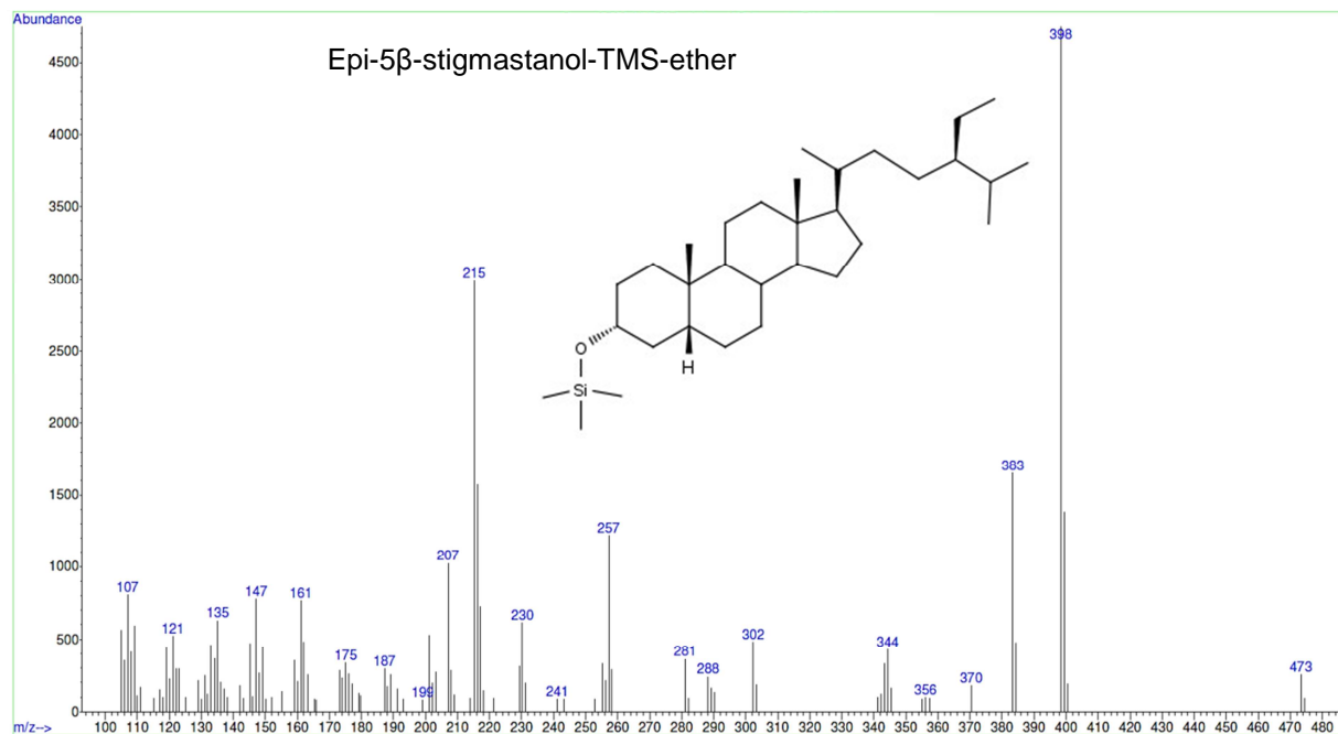
S16 Fig. Mass spectrum and structural formula of epi-5 \beta -stigmastanol trimethylsilyl ether.
