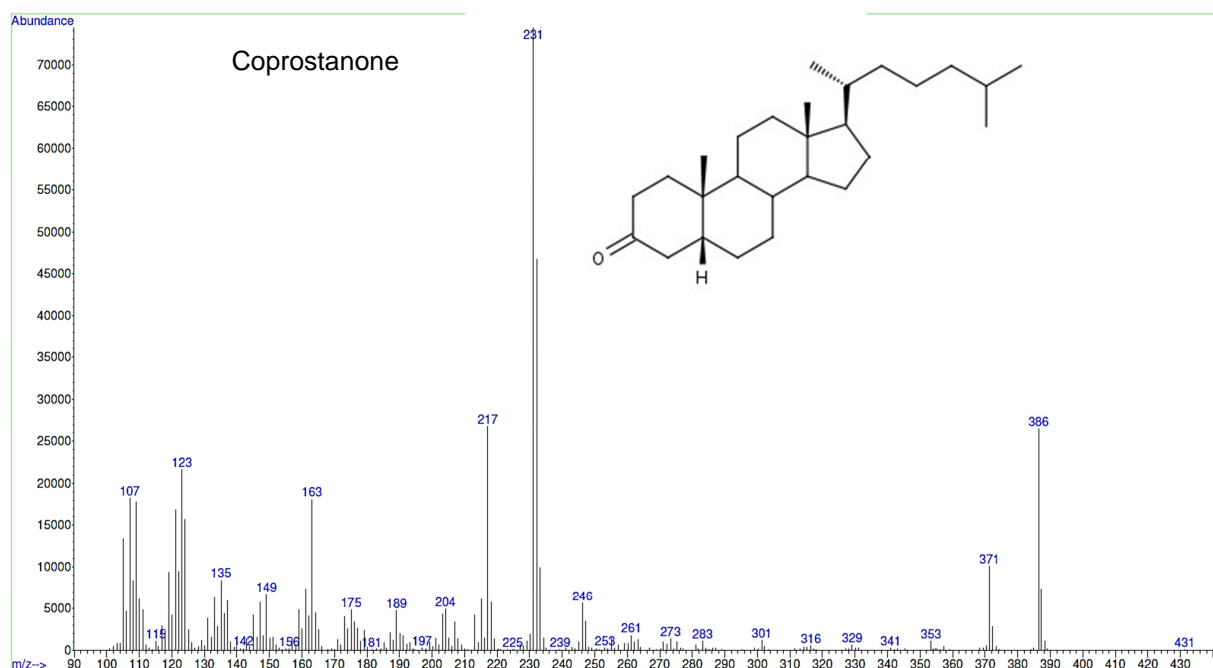
S18 Fig. Mass spectrum and structural formula of coprostanone.
