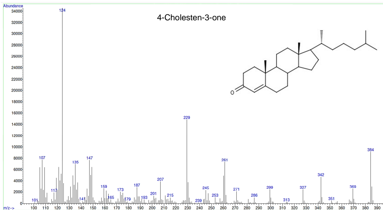
S19 Fig. Mass spectrum and structural formula of 4-cholesten-3-one.
