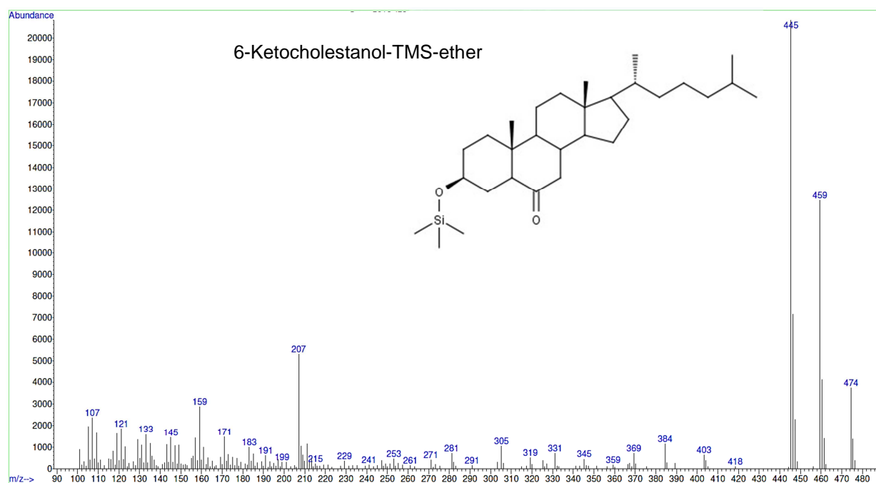
S20 Fig. Mass spectrum and structural formula of 6-ketocholestanol trimethylsilyl ether.
