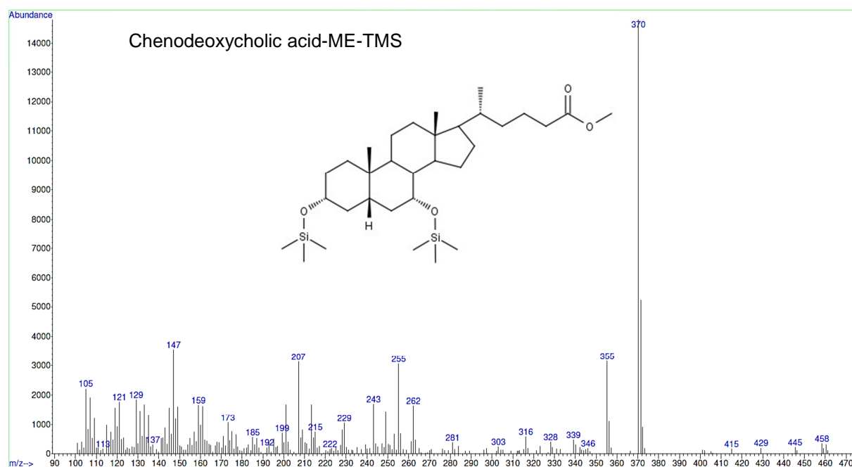
S21 Fig. Mass spectrum and structural formula of methylated and silylated chenodeoxycholic acid.
