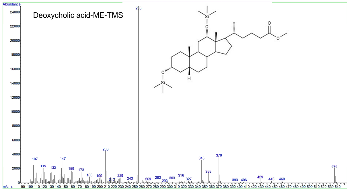
S22 Fig. Mass spectrum and structural formula of methylated and silylated deoxycholic acid.
