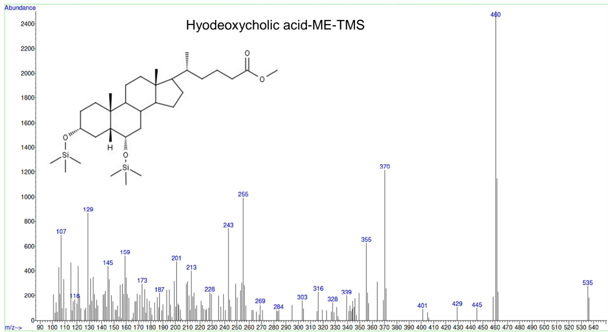
S23 Fig. Mass spectrum and structural formula of methylated and silylated hydoxycholeic acid.
