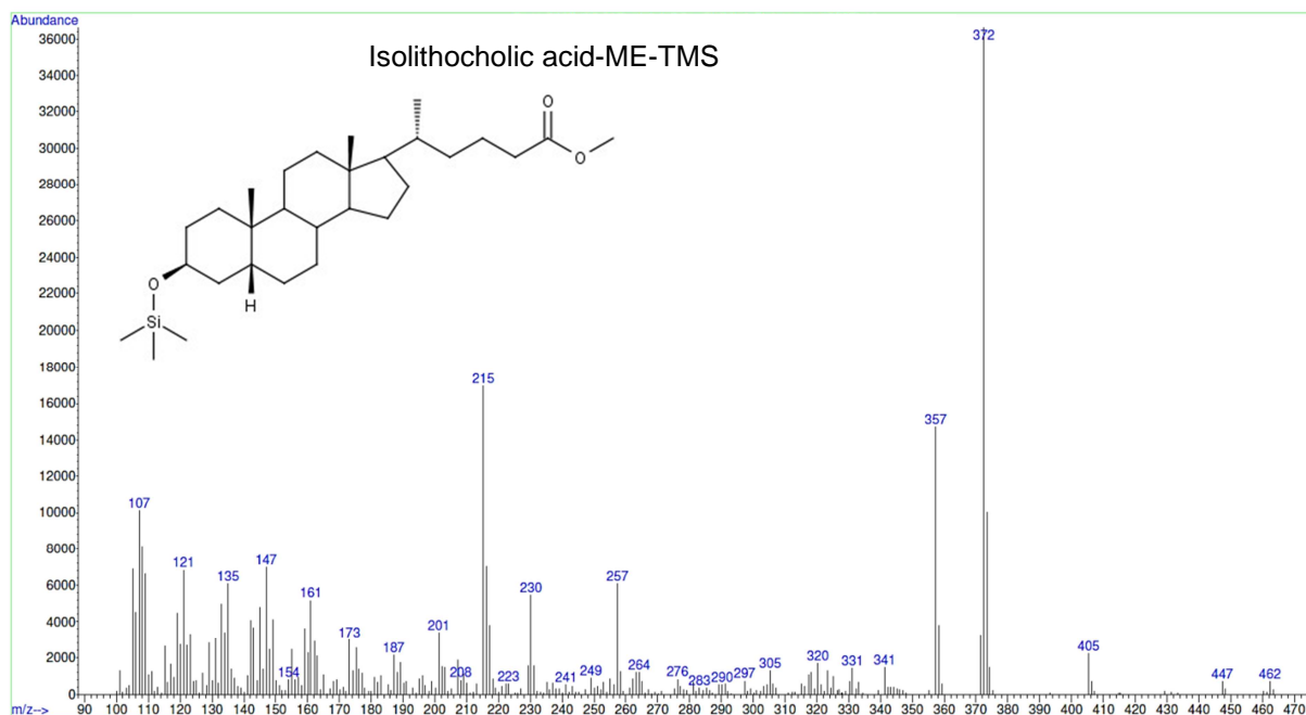
S24 Fig. Mass spectrum and structural formula of methylated and silylated isolithocholic acid.
