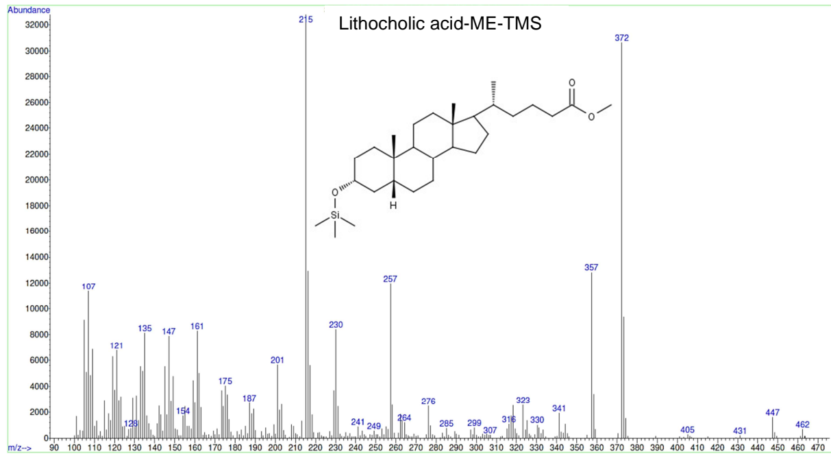
S25 Fig. Mass spectrum and structural formula of methylated and silylated lithocholic acid.
