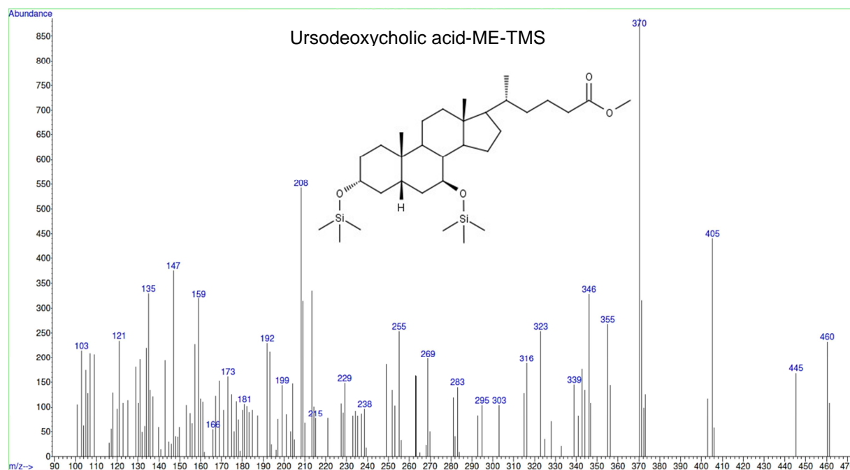
S26 Fig. Mass spectrum and structural formula of methylated and silylated ursodeoxycholic acid.
