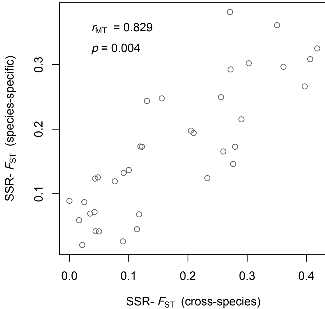
Additional file 10: Figure S6 Comparison of pairwise population genetic differentiation ( F_{ST} ) among nine populations of Arabidopsis halleri based on 12 cross-species microsatellite markers and seven species-specific microsatellite markers. r_{MT} represents the correlation coefficient of the Mantel test and p the significance of the correlation.
