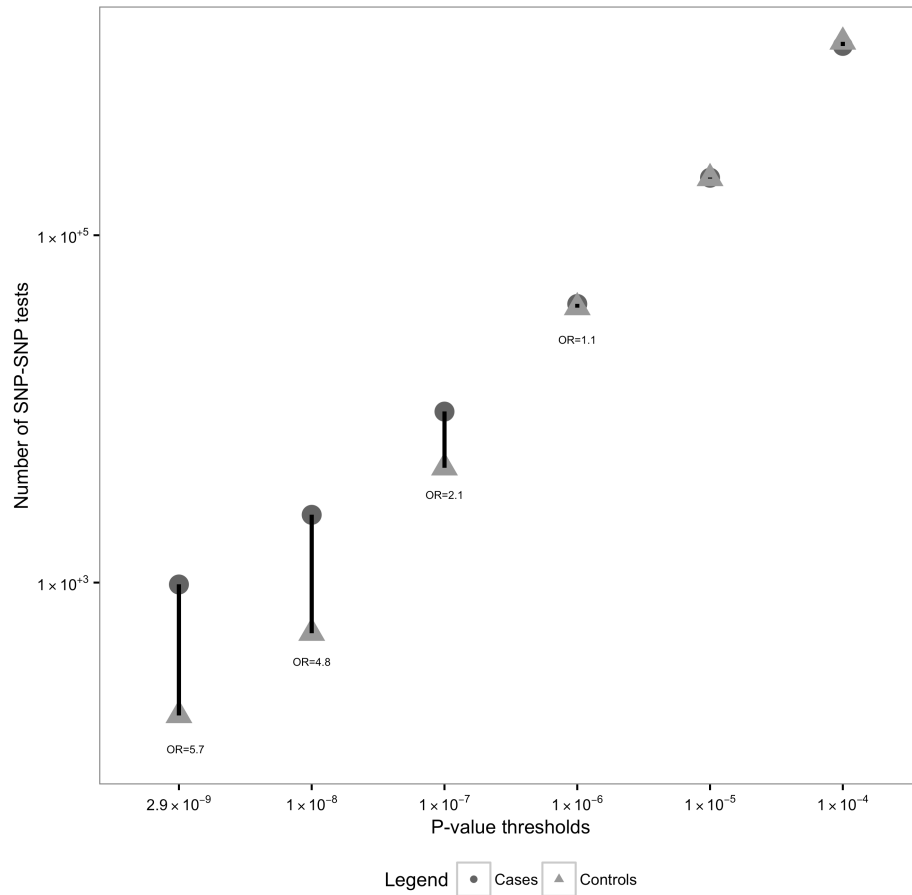
Figure S3. Epistasis in sibling-paired SSC dataset. The graph displays the number of epistasis tests (y-axis) in the ASD cases (dark gray, circle) and unaffected matched siblings (light gray, triangle) with P -value below thresholds (x-axis, left to right): P < 2.9 \times 10^{-9} , P < 1.0 \times 10^{-8} , P < 1.0 \times 10^{-7} , P < 1.0 \times 10^{-6} , P < 1.0 \times 10^{-5} , and P < 1.0 \times 10^{-4} . The 2x2 chi-square test odds ratio (OR) is written for the epistasis results meeting nominal significance ( P < 10^{-6} ).
