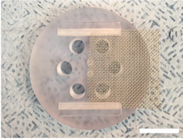
SUPPLEMENTARY FIG. S1. Scaffold holder and support mesh. Six scaffolds of 8 mm in diameter were distributed axi-symmetrically within a custom-made polycarbonate holder. A support mesh made of stainless steel 316 slides into place to prevent the movement of scaffolds during flow perfusion culture. Scale bar represents 2 cm.
