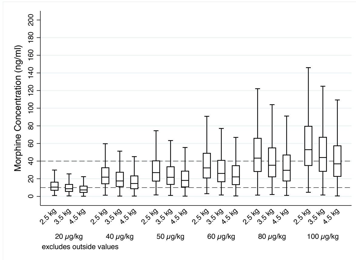
Supplemental Figure S1. Predicted morphine trough concentrations with different intermittent morphine doses given every 6 hours by birthweight. Each boxplot represents steady-state trough concentrations from 1000 simulated neonates with HIE receiving hypothermia. Outliers are not presented. Dashed lines reference target concentrations between 10 to 40 ng/ml.
