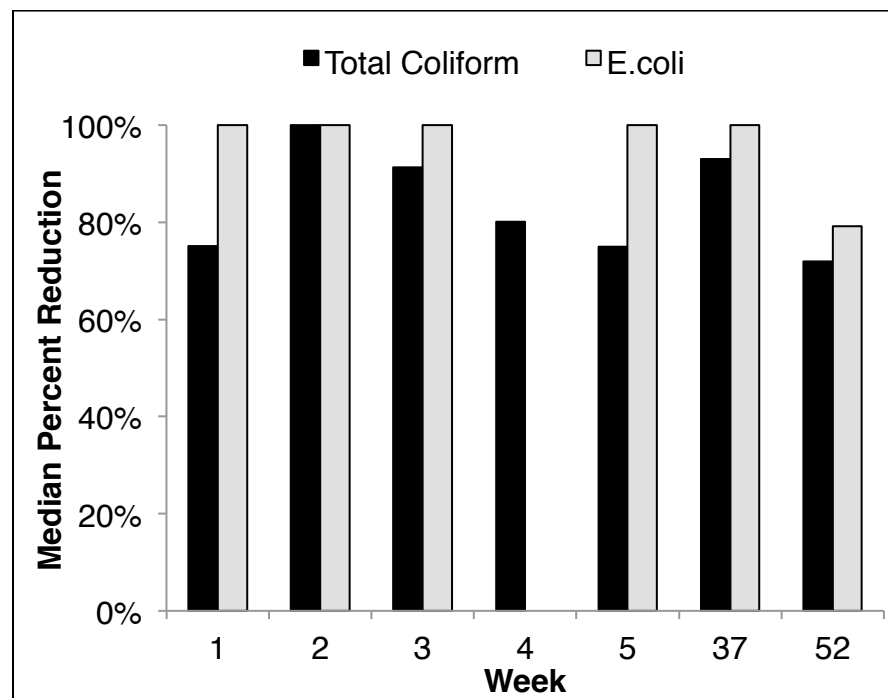
S8 Fig. Median percent reduction of total coliform bacteria and E. coli among ceramic tablet treated samples. Percent reduction was determined by comparing bacteria levels in water storage containers treated with control ceramic tablets to those treated with silver-embedded ceramic tablets. Samples were taken in duplicate among 29 households over 12 months. Data points represent the median of all samples.
