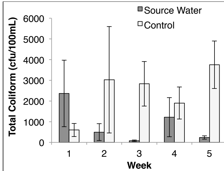
S11 Fig. Total coliform bacteria levels at the water source and in water storage containers at the household level over time.
