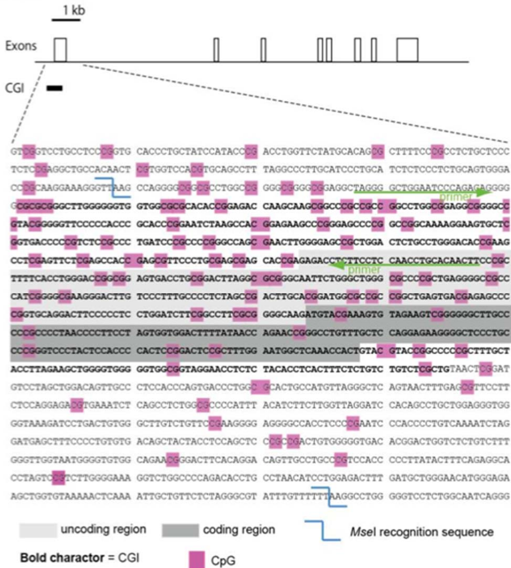
Figure S1. The detailed structure of CpG island in RAR \alpha promoter. Bold characters indicate CpG island (CGI) and pink squares indicate CpG. The primers used in Figure 5A are presented by green arrows.
