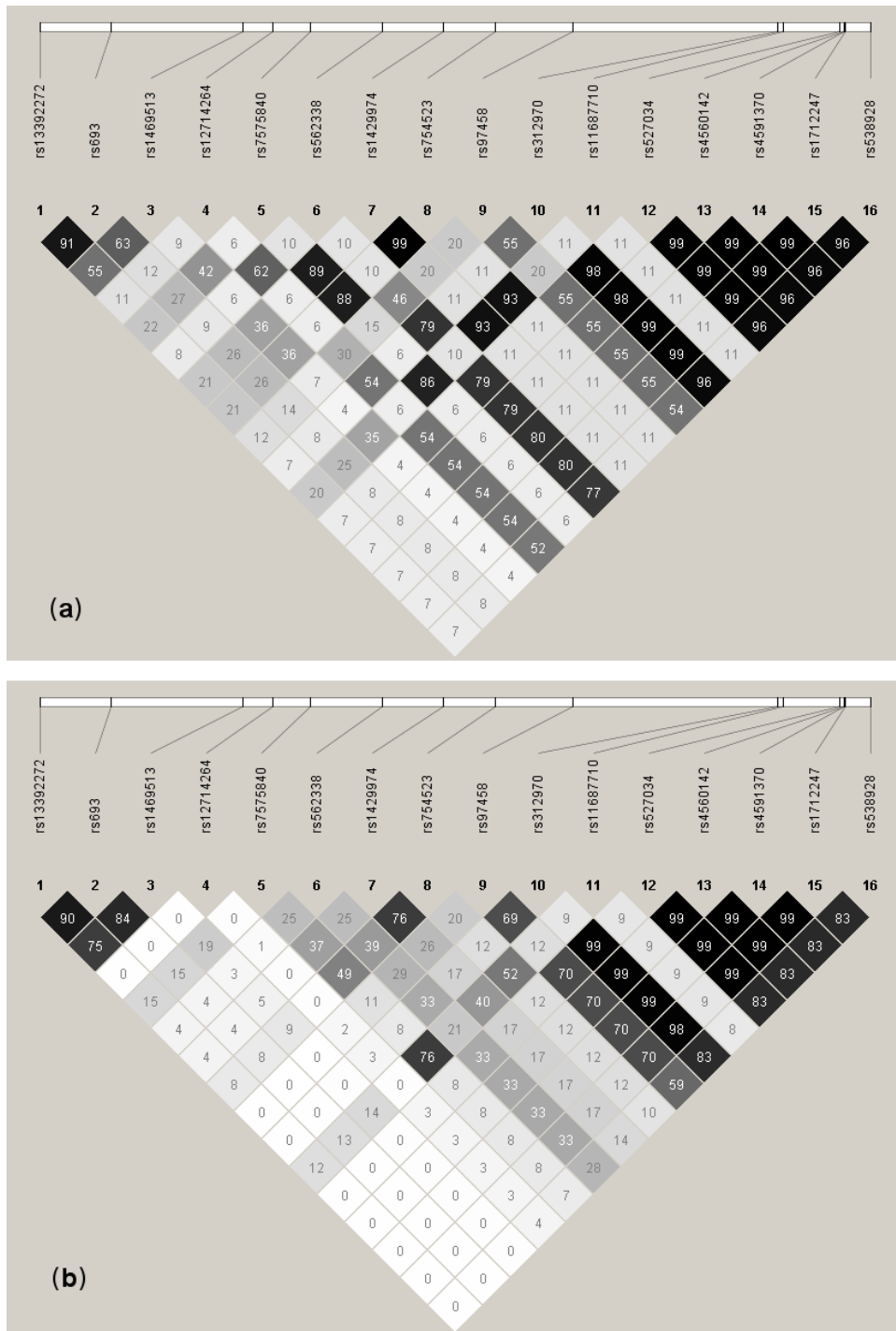
Figure S1. Linkage disequilibrium (LD) patterns.
