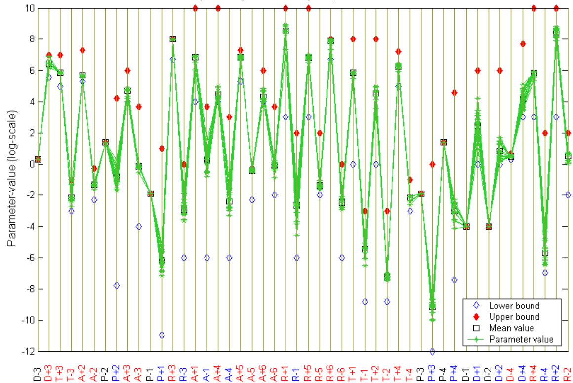
Cobweb plot using 16 different good parameter-value sets
