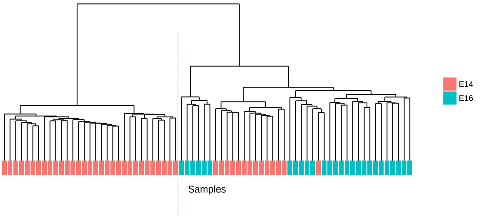
Dendrogram of Hierarchical Clustering (Euclidean + Ward) on Treutlein et al.
