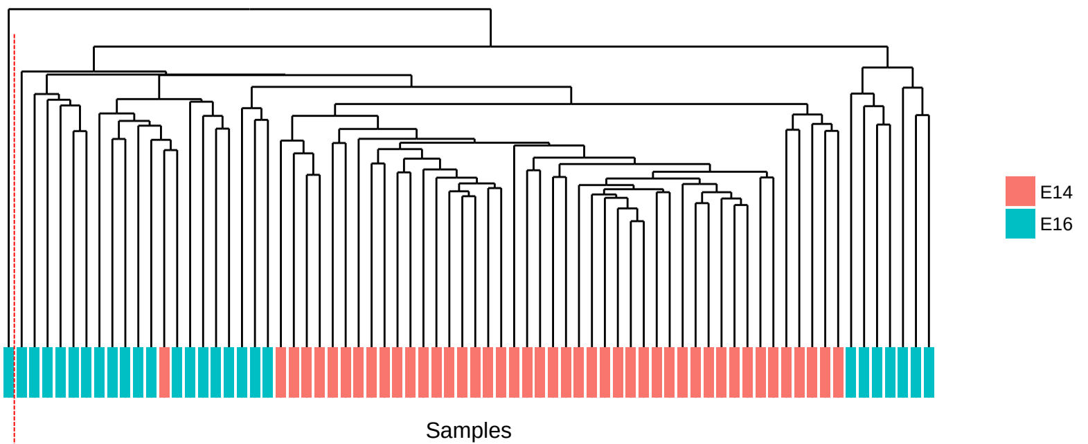
Dendrogram of Hierarchical Clustering (Correlation + Complete) on Treutlein et al.
