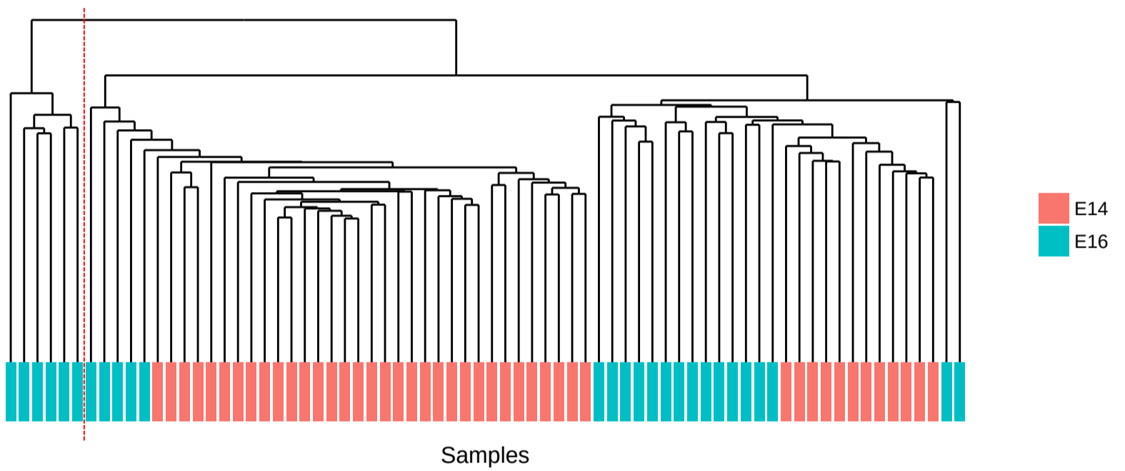
Dendrogram of Hierarchical Clustering (Euclidean + Complete) on Treutlein et al.
