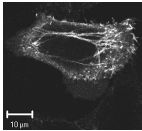
GFP-PLCδ(PH)
