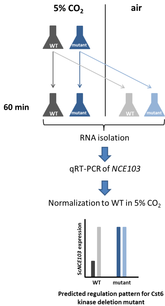
Fig. S2 Workflow of mutant library screening for Cst6 kinase identification
