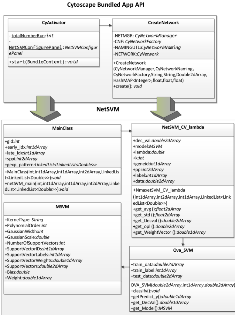
S2 Fig. The class diagram of the CyNetSVM bundle application
