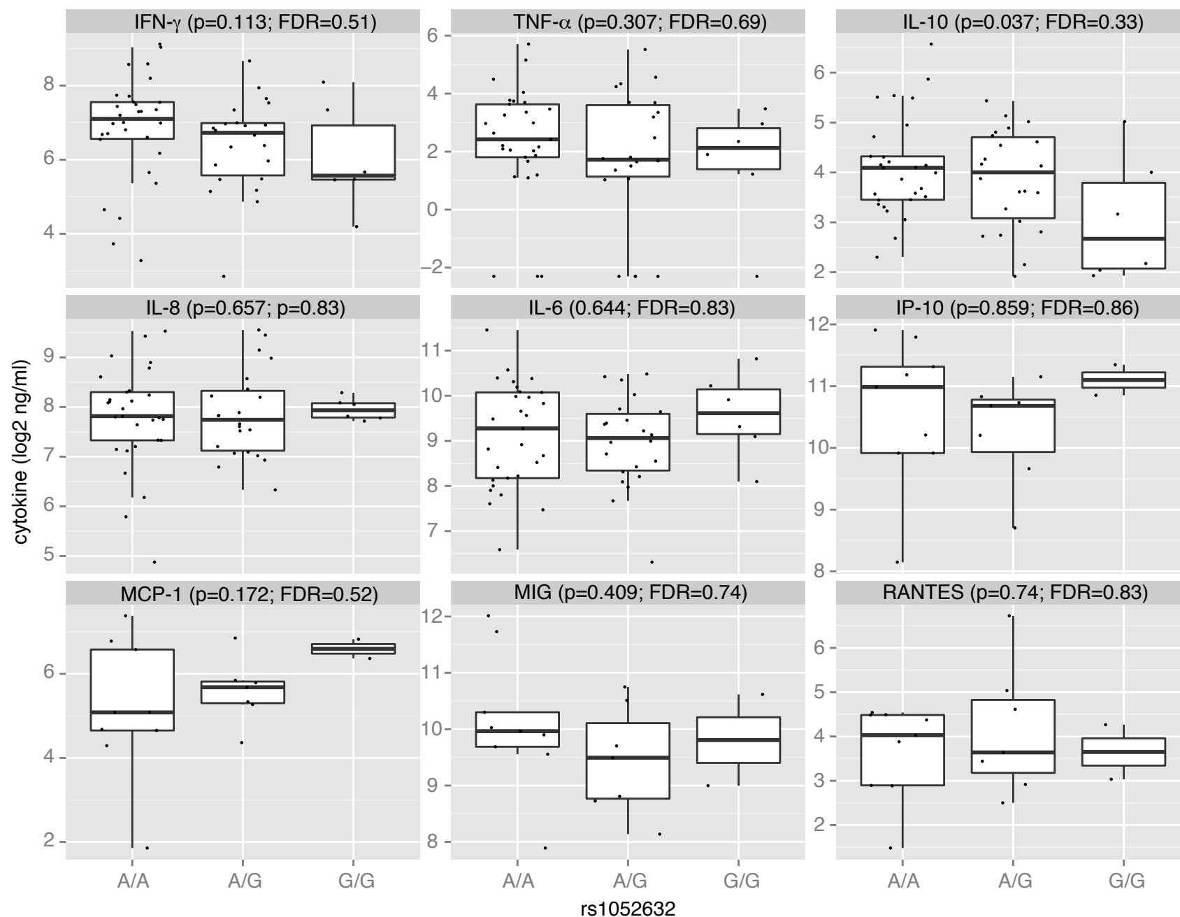
Supplementary Figure 1. Analysis of cytokines in the CSF of patients with tuberculous meningitis. CSF from patients with meningeal tuberculosis were analyzed for the presence of inflammatory or regulatory cytokines by multiplex bead array (Luminex). Raw cytokine values were log 2 transformed and generalized linear regression was used to determine the association with rs1052632 genotype. Shown are the p-value of the association and correction of the false discovery rate (FDR) per the Benjamini-Hochberg method.
