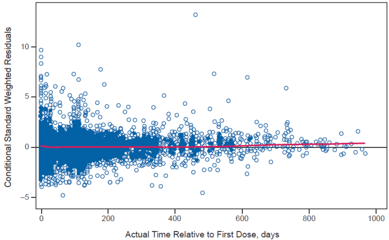
Supplemental Figure S1. Final model. Conditional weighted residuals with interaction (CWRESI) versus actual time after first dose.
