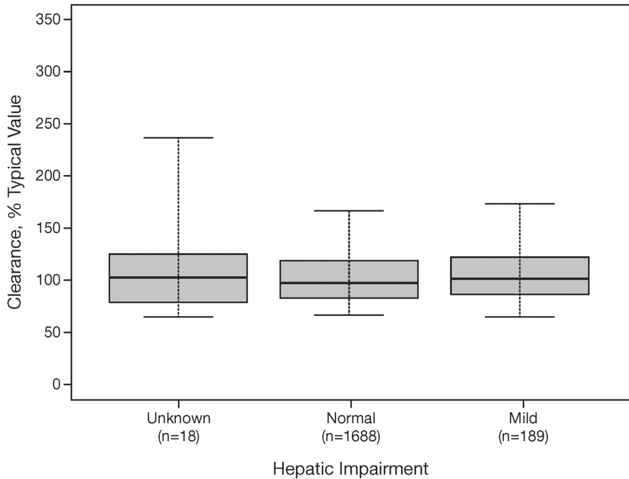
Supplemental Figure S6. Box plots showing the apparent lack of relationship between hepatic function status and nivolumab clearance.
