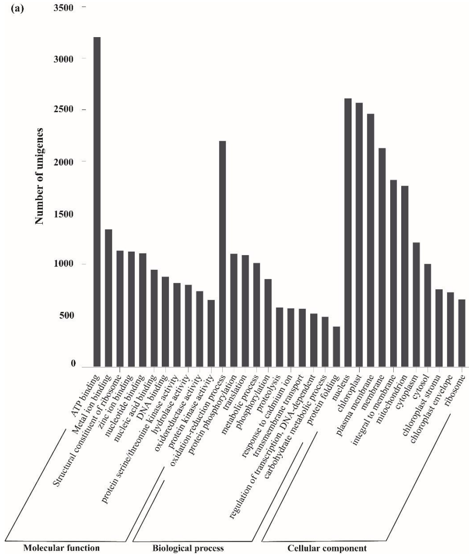
Additional file 2 (a) Functional annotation of the assembled unigenes based on GO category, the functions of the unigenes were divided into three categories. (b) Information of clusters of orthologous groups (COG) classification, the unigenes were mainly clustered into 25 components.
