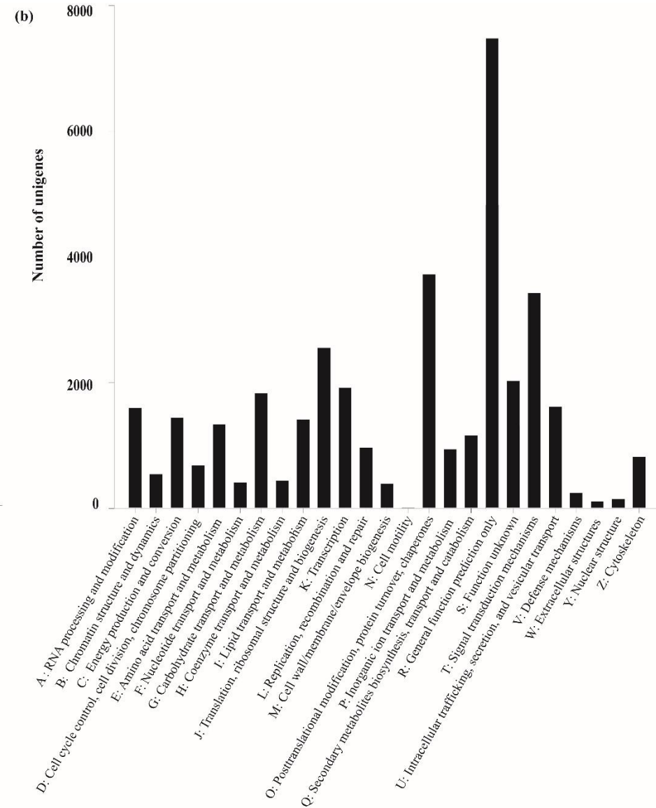
Additional file 2 (a) Functional annotation of the assembled unigenes based on GO category, the functions of the unigenes were divided into three categories. (b) Information of clusters of orthologous groups (COG) classification, the unigenes were mainly clustered into 25 components.
