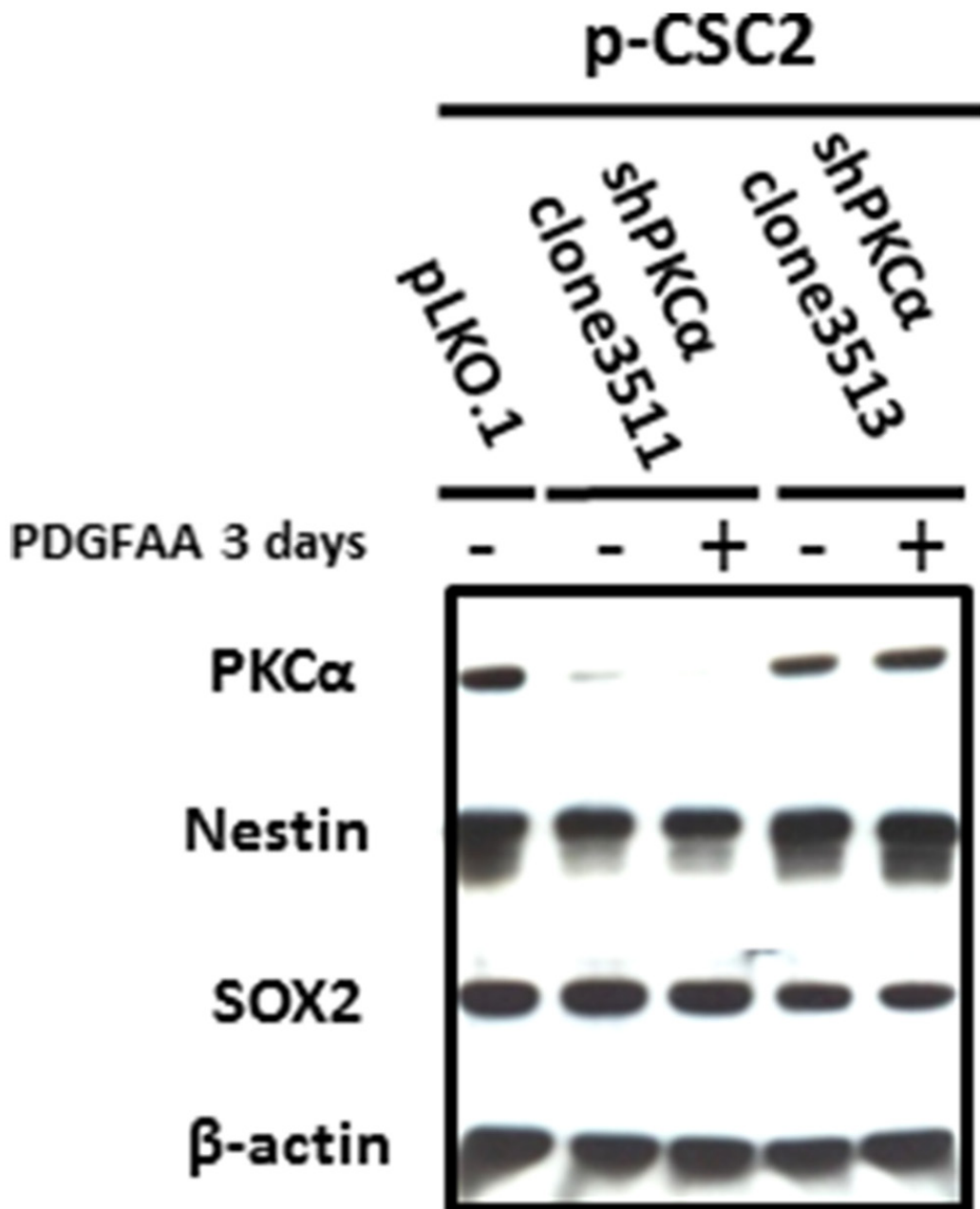
Supplementary Figure S1: PKC \alpha is not involved in the regulation of stemness in p-CSC2. Reduction of PKC \alpha protein expression in shPKC \alpha cell clones does not affect expression of multipotency stem cell markers Nestin and Sox2 compared to pLKO.1 cell, after 3 days of PDGF-AA treatment.
