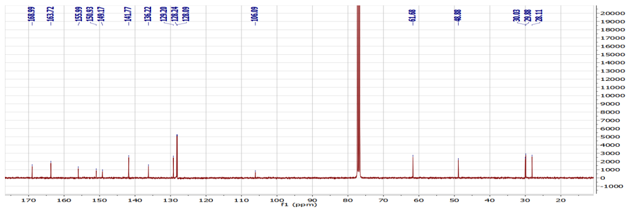
13 C-RMN spectra of 6a
