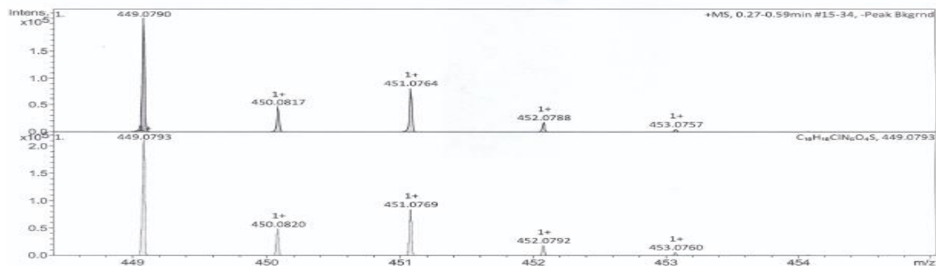
HRMS spectra of 6c
