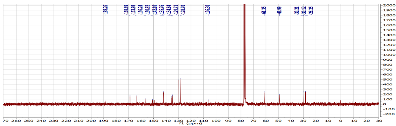
13 C-RMN spectra of 6c
