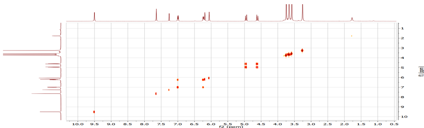
2D-COSY spectra of 6i
