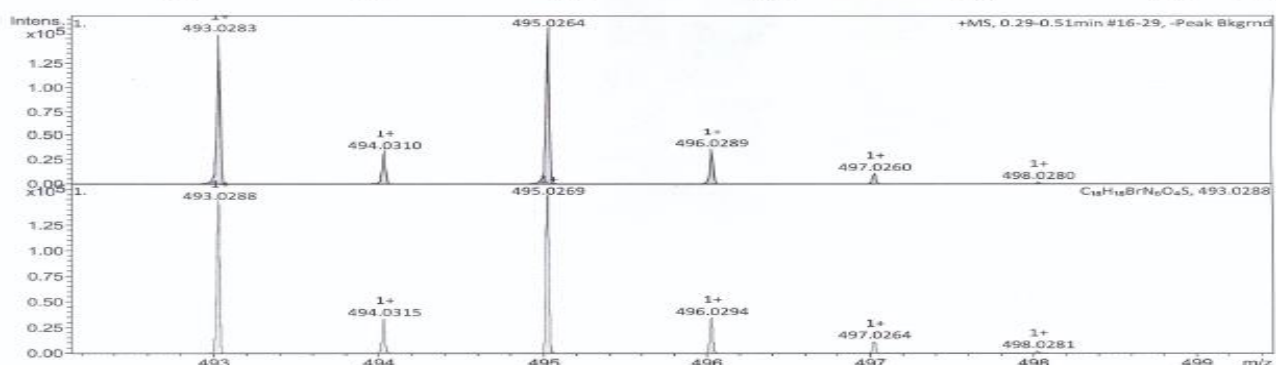
HRMS spectra of 6b
