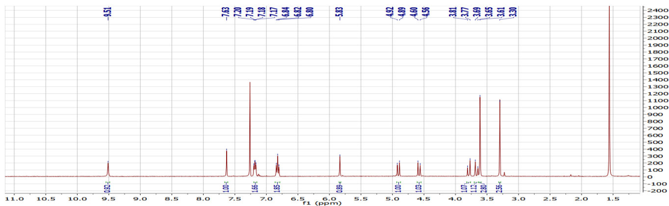
1 H-RMN spectra of 6d
