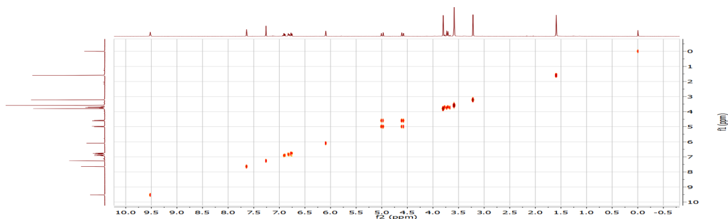
2D-COSY spectra of 6h
