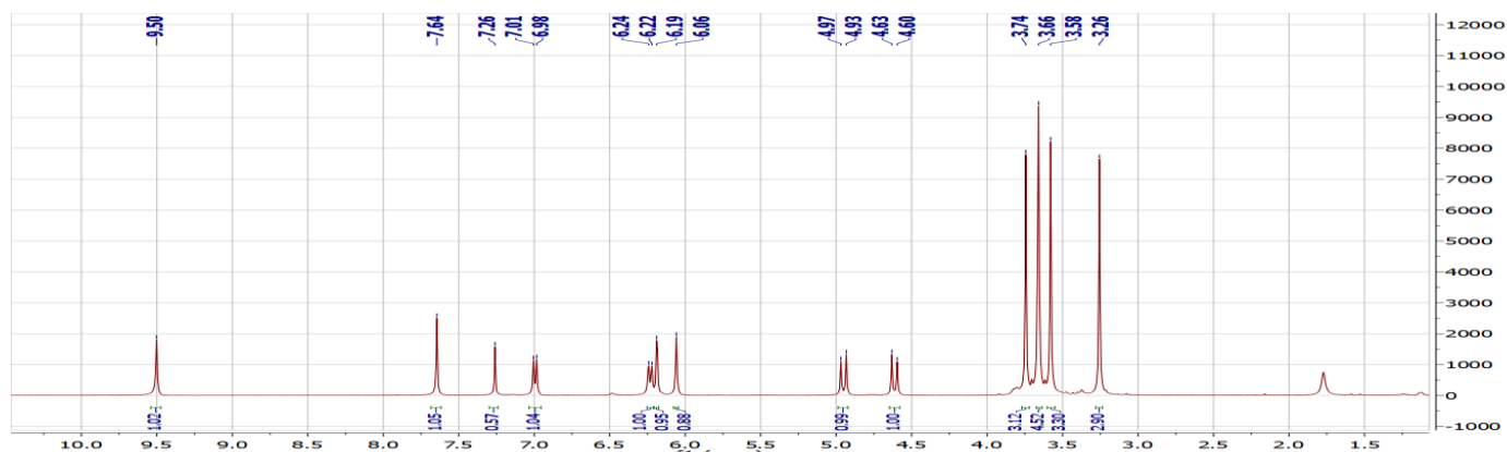
1 H-RMN spectra of 6i
