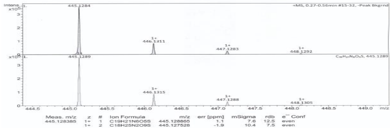
HRMS spectra of 6e
