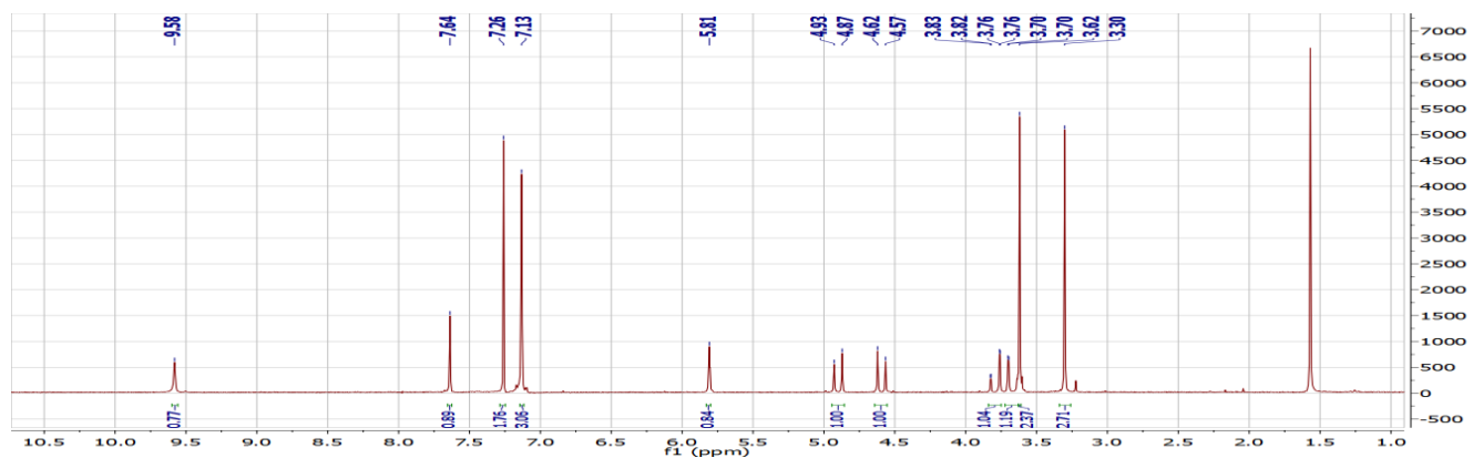
1 H-RMN spectra of 6c
