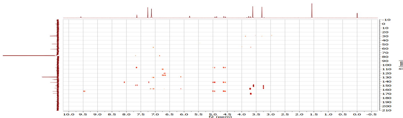
HMBC spectra of 6c
