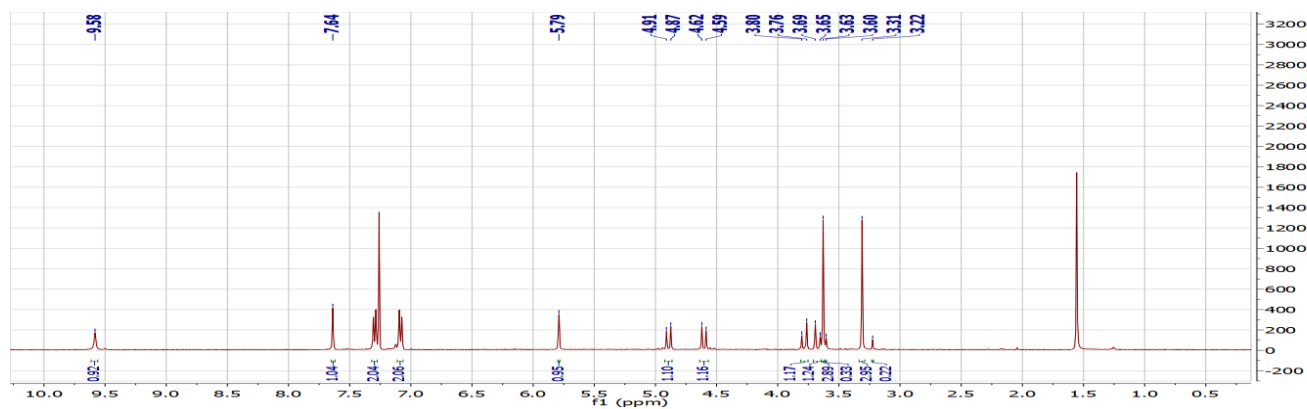
1 H-RMN spectra of 6b
