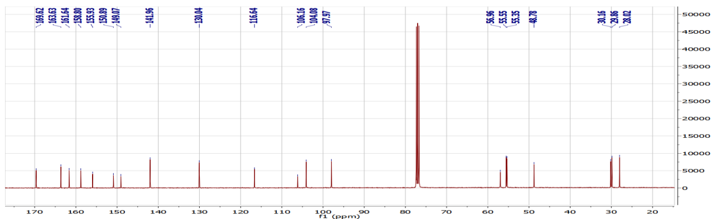
13 C-RMN spectra of 6i
