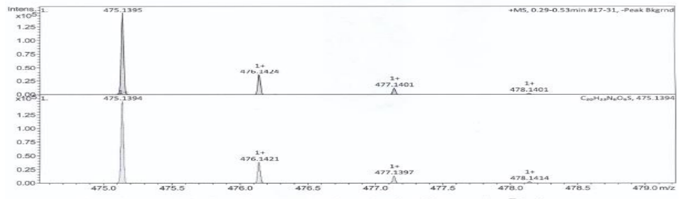
HRMS spectra of 6h
