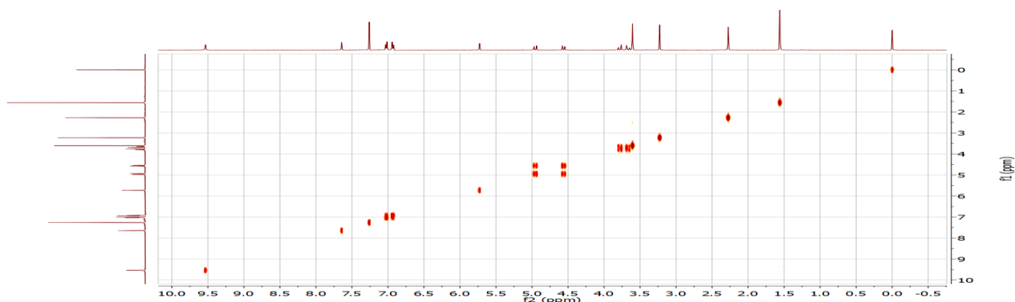
2D-COSY spectra of 6k
