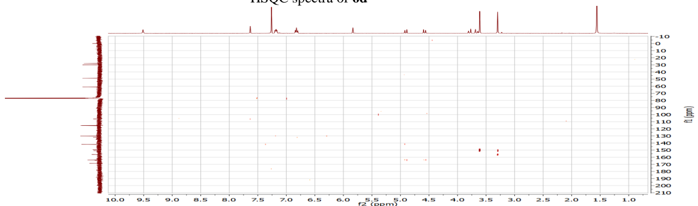
HMBC spectra of 6d
