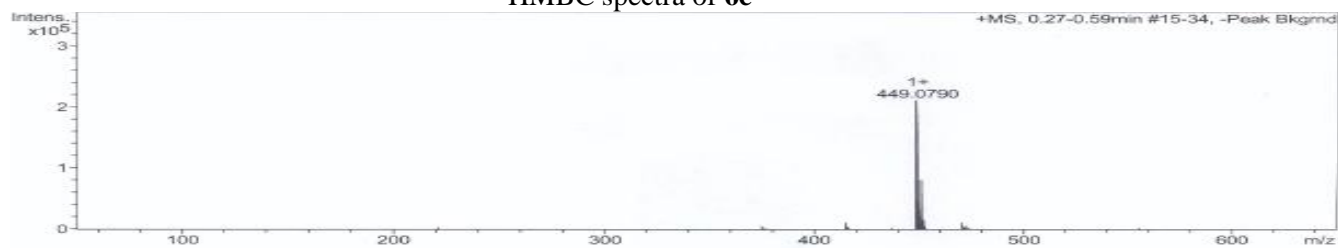
HMBC spectra of 6c
