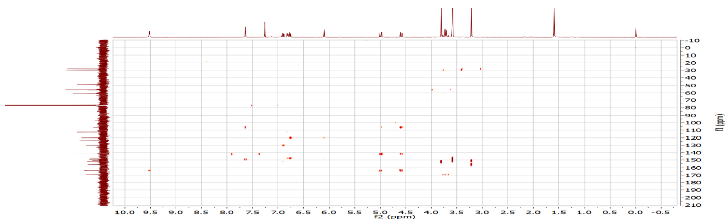
HMBC spectra of 6h
