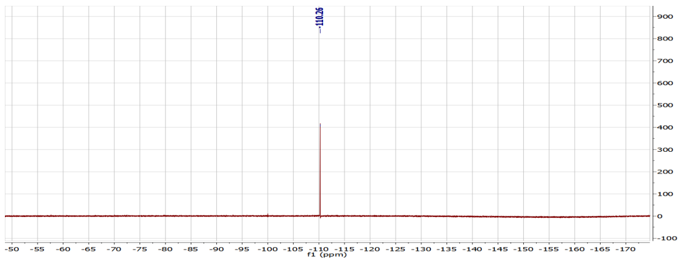
^{19}\text{F} -RMN spectra of 6f
