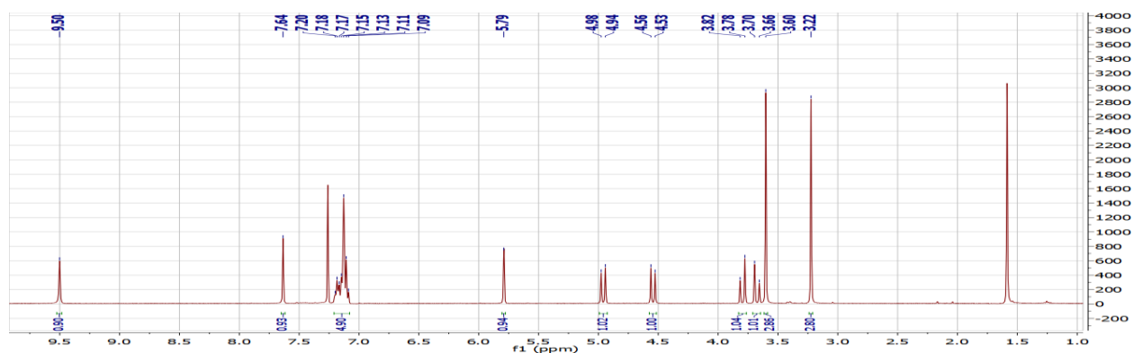
1 H-RMN spectra of 6a
