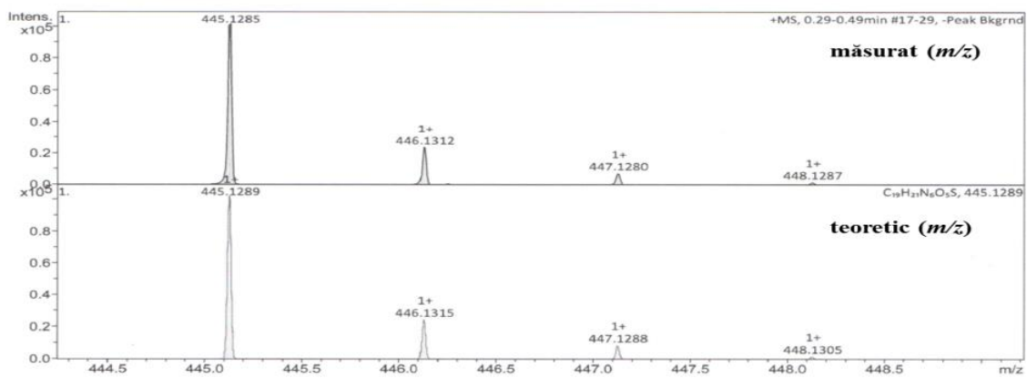
HRMS spectra of 6k
