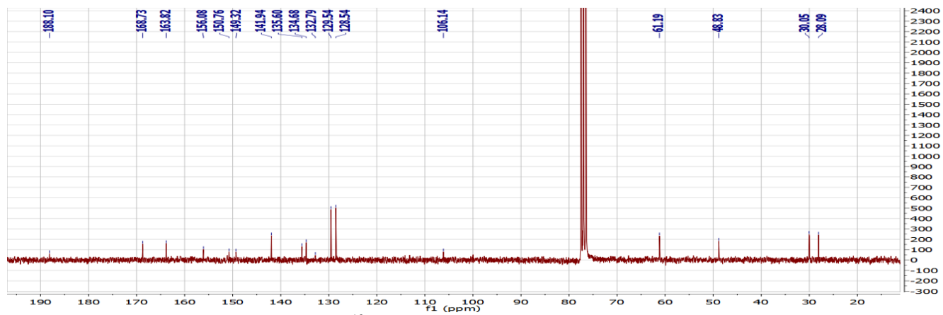
13 C-RMN spectra of 6b
