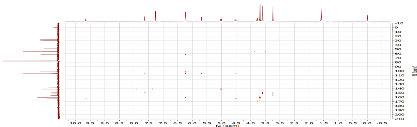
HMBC spectra of 6j
