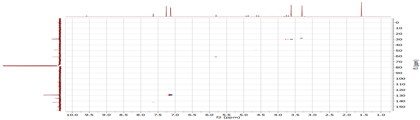
HSQC spectra of 6c
