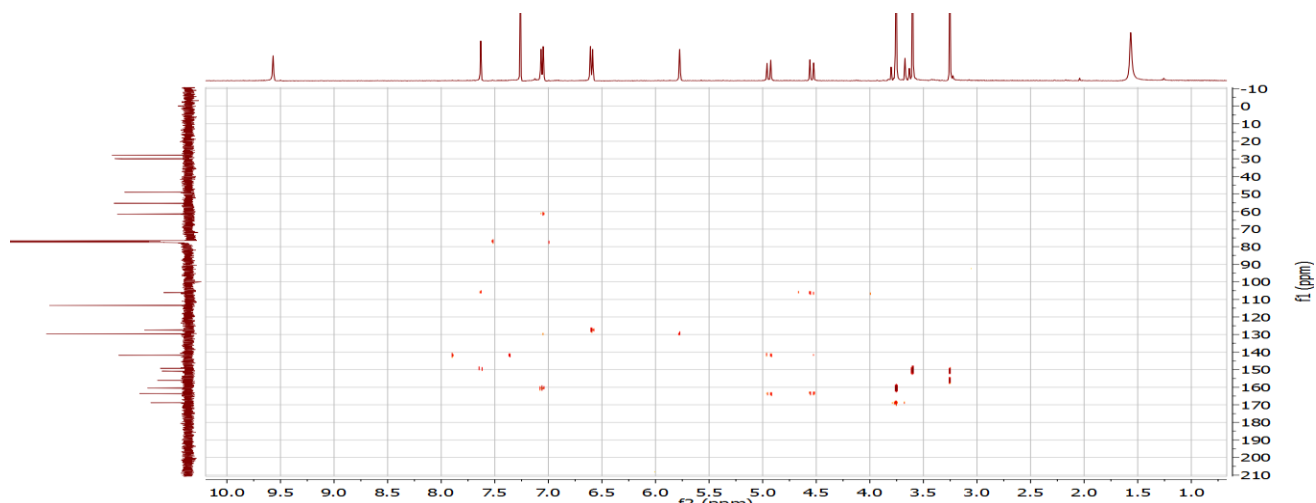
HMBC spectra of 6f
