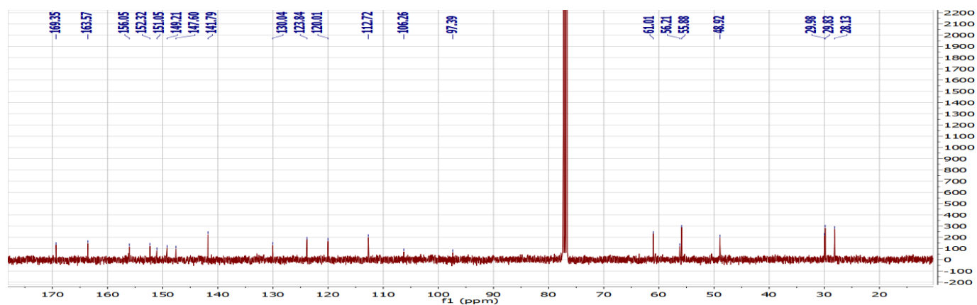
13 C-RMN spectra of 6h
