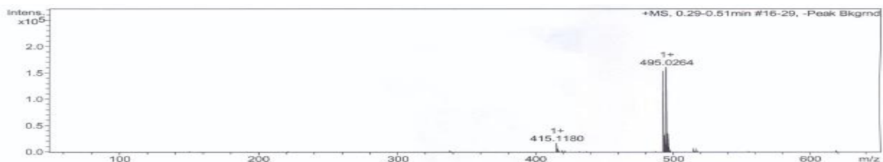
HMBC spectra of 6b
