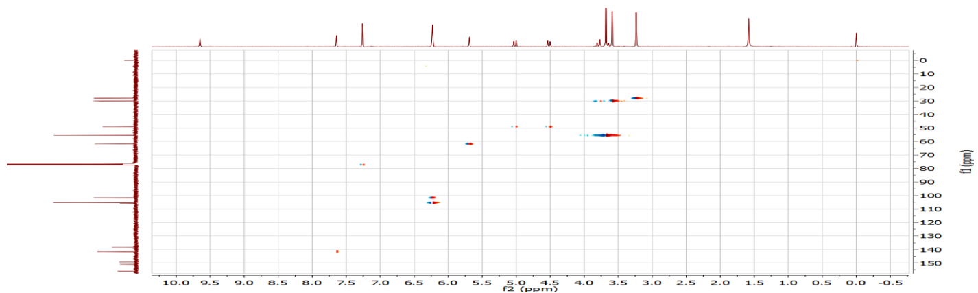
HSQC spectra of 6j
