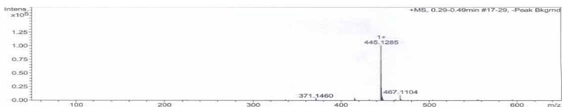
HMBC spectra of 6f
