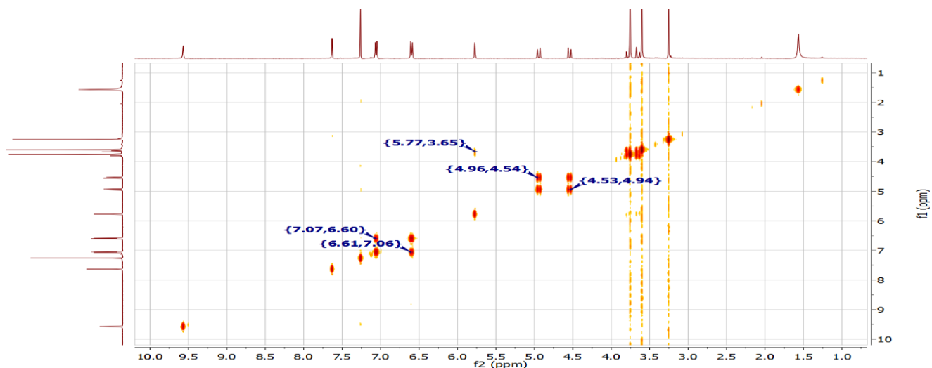
2D-COSY spectra of 6f
