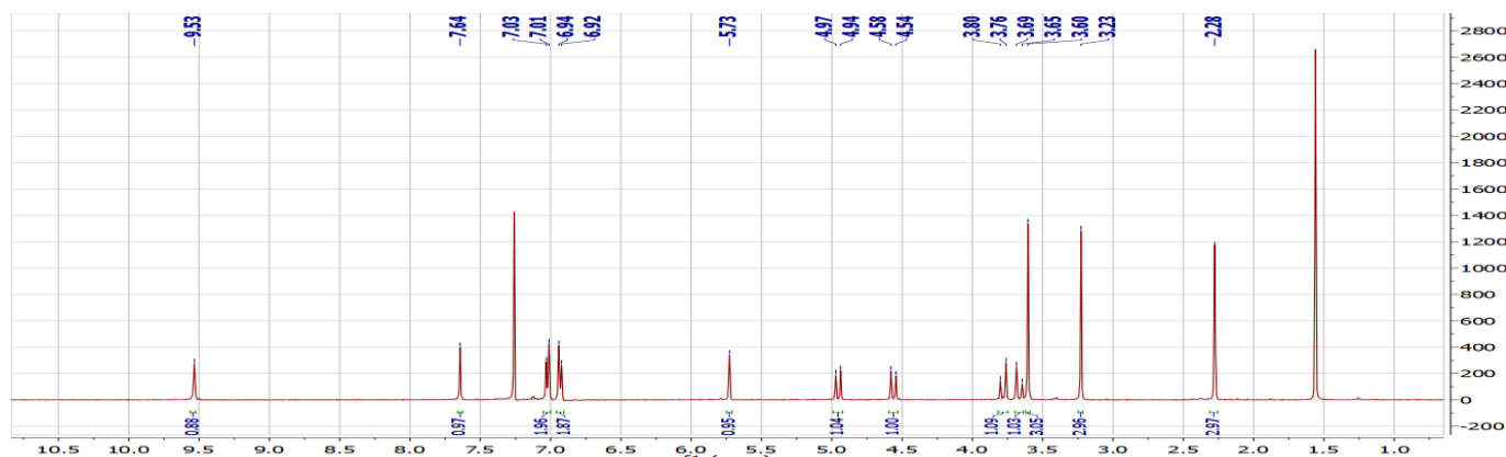
1 H-RMN spectra of 6k
