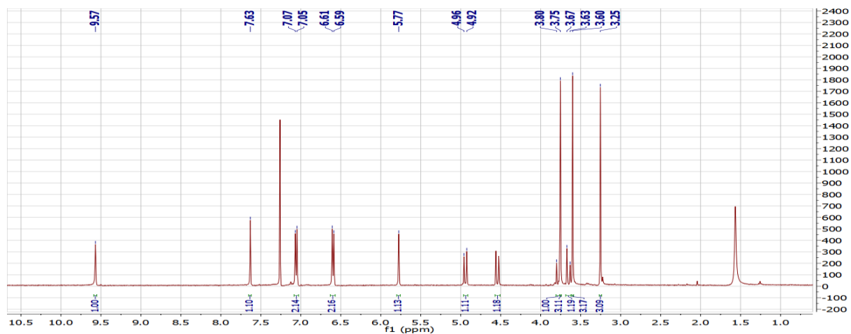
1 H-RMN spectra of 6f
