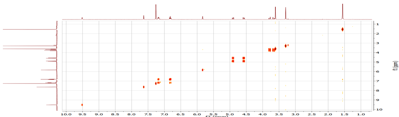
2D-COSY spectra of 6d
