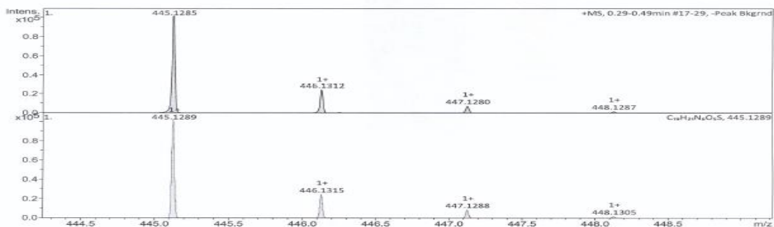
HRMS spectra for 6f
