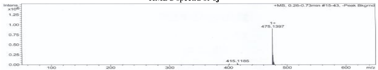
HMBC spectra of 6j
