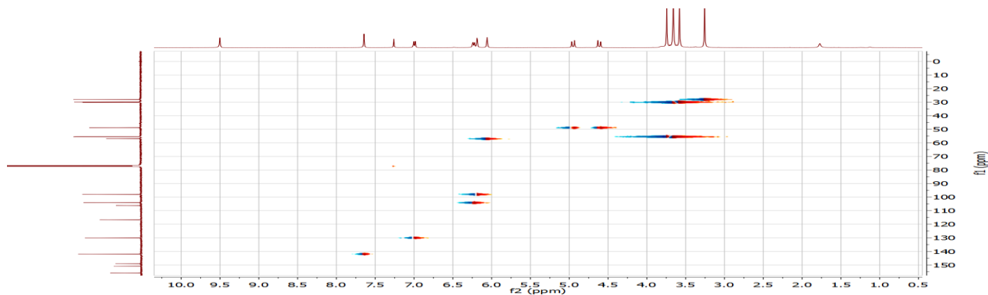
HSQC spectra of 6i
