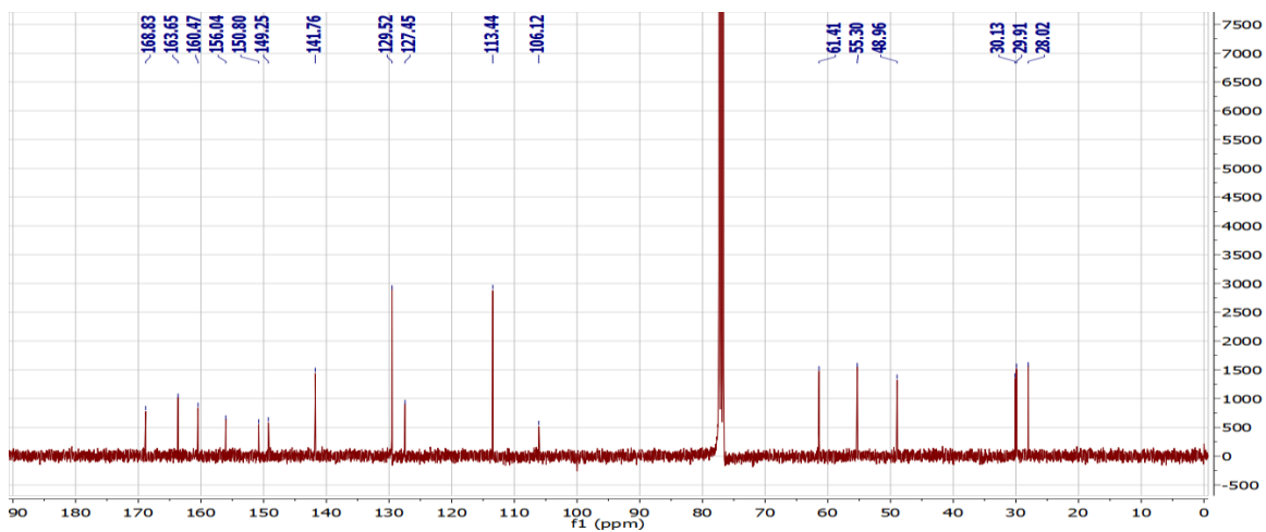
13 C-RMN spectra of 6f
