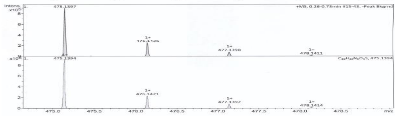
HRMS spectra of 6j
