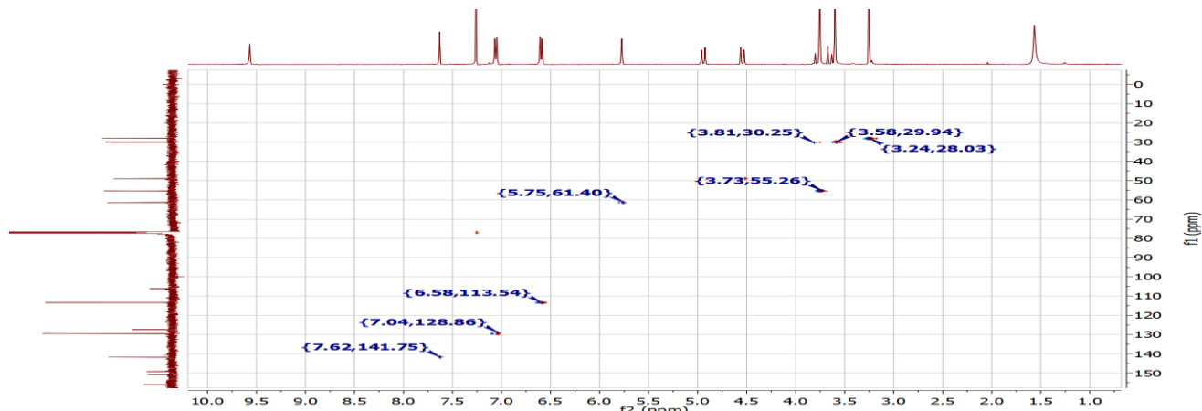
HSQC spectra of 6f
