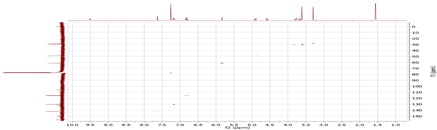
HSQC spectra of 6d
