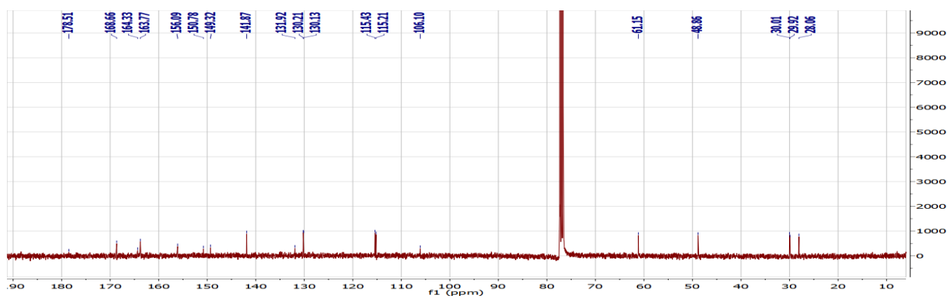
13 C-RMN spectra of 6d
