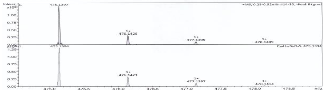
HRMS spectra of 6i
