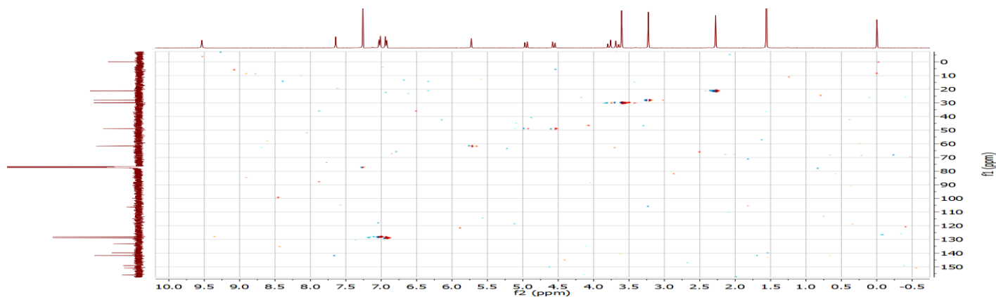
HSQC spectra of 6k
