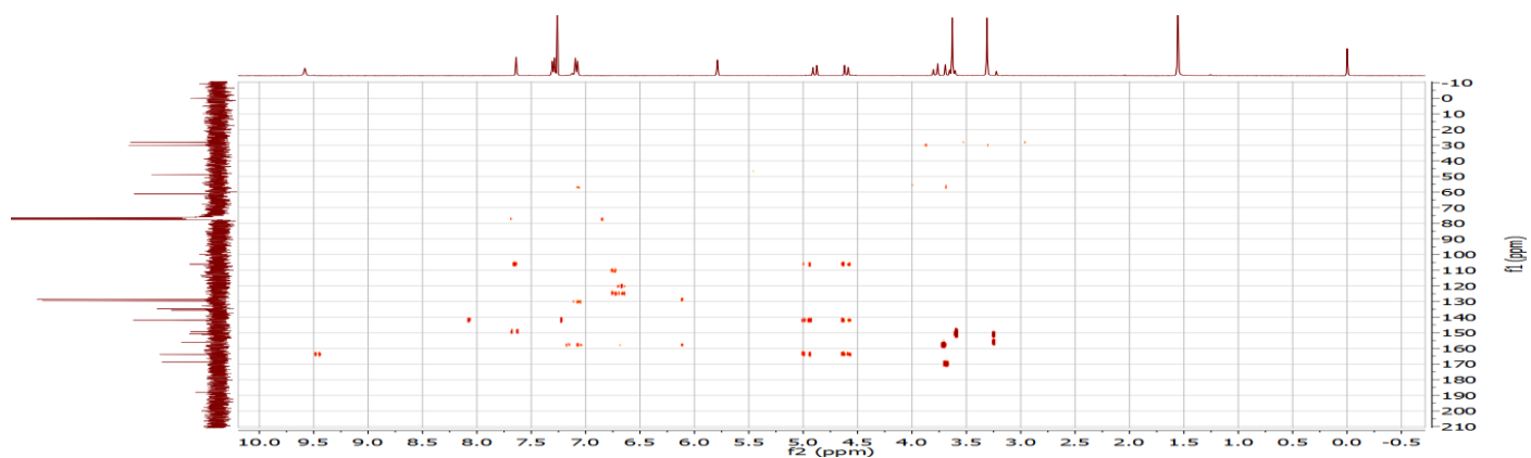
HMBC spectra of 6b
