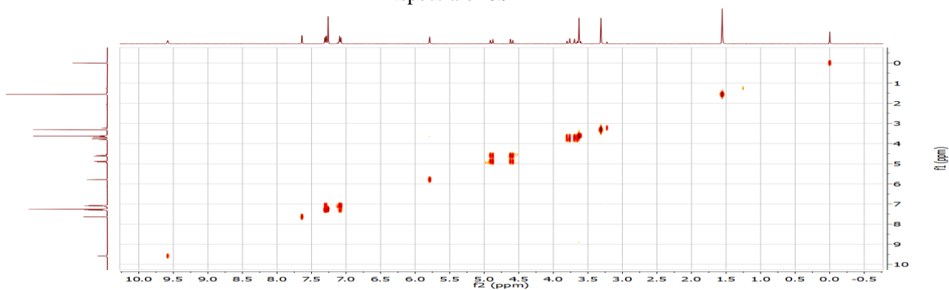
2D-COSY spectra of 6b
