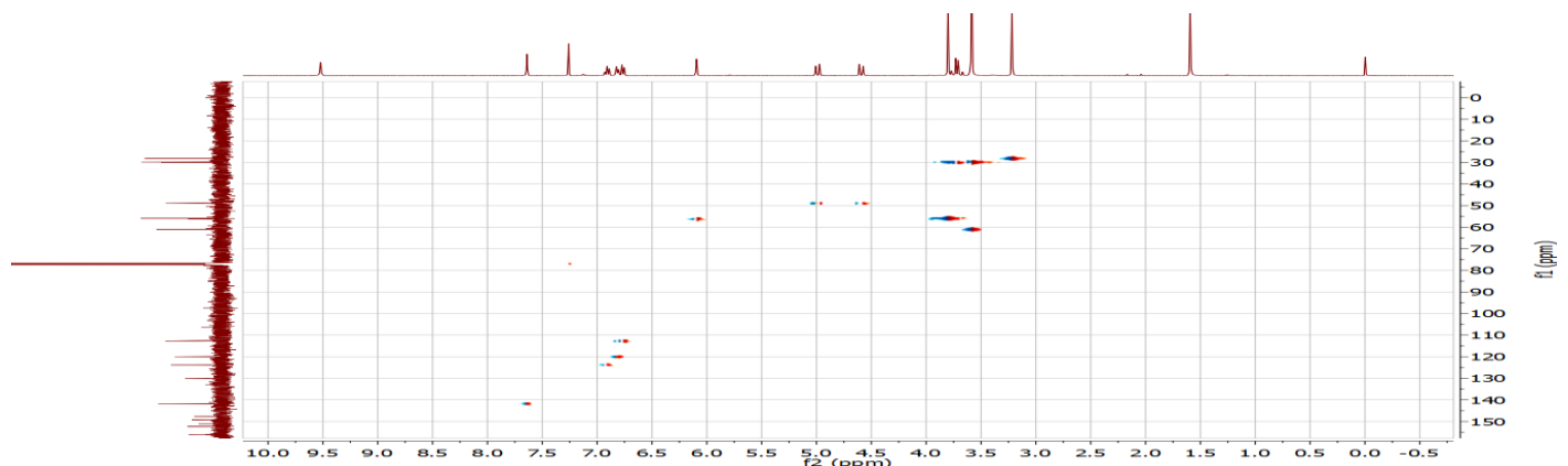
HSQC spectra of 6h
