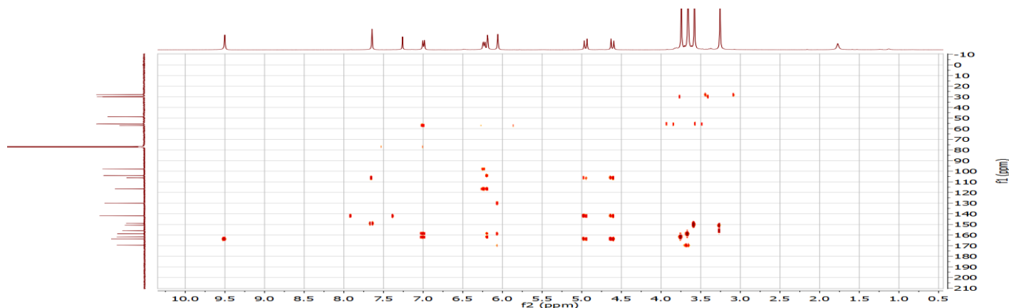
HMBC spectra of 6i
