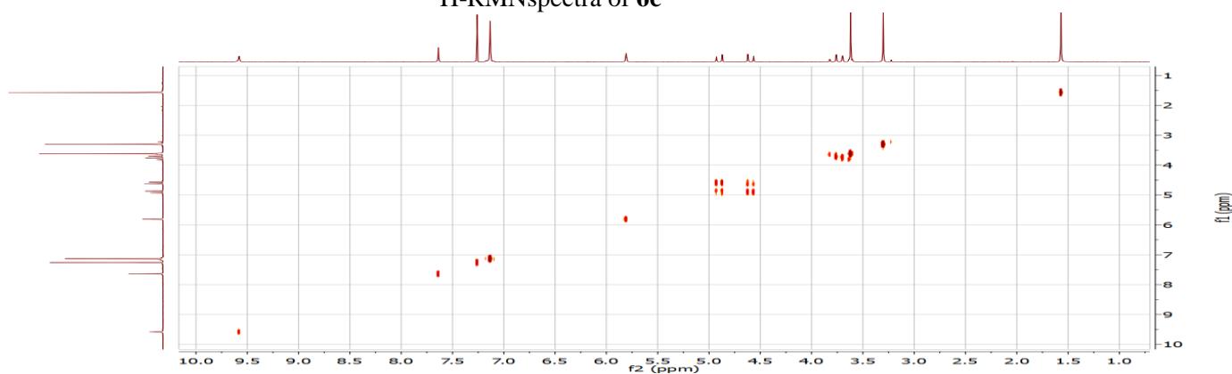
2D-COSY spectra of 6c
