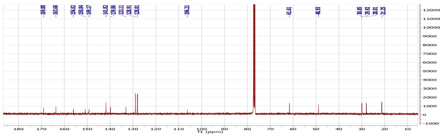
13 C-RMN spectra of 6k
