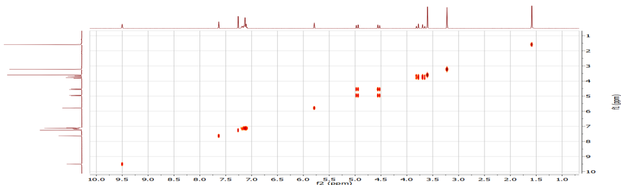
2D-COSY spectra of 6a
