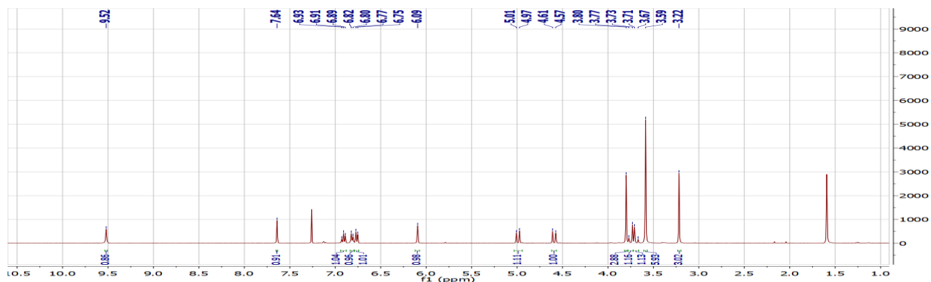
1 H-RMN spectra of 6h
