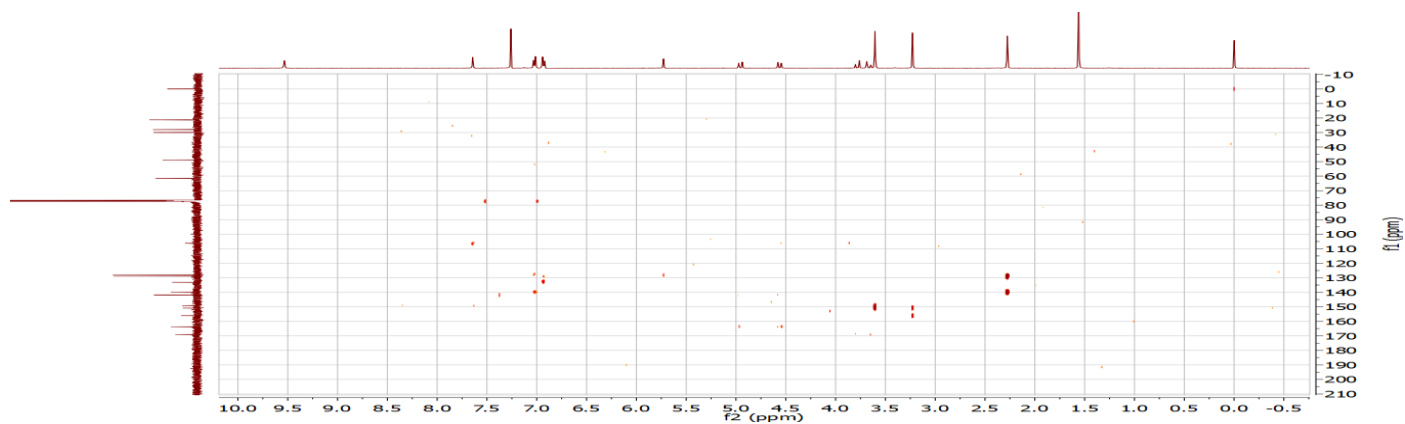
HMBC spectra of 6k
