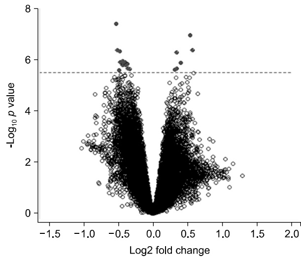
Supplementary Fig. 3. Volcano plot for differential gene expression profiles between autism spectrum disorders (ASDs) and controls. The blue line represents p value at family wise error rate of 0.05 ( -\log_{10}p=5.5 ). The red dots represent probes significantly differentially expressed between subjects with ASD (n=13) and controls (n=13) from the training set.
