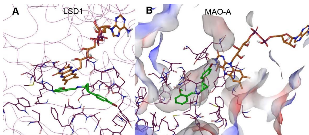
Figure S1. Docking results of compound 26 (as tube models with C atoms in green). (A) The lowest-energy docking structure in the active site of LSD1; and (B) The lowest-energy docking structure in the active site of MAO-A, showing selected interacting amino acid residues (with C atoms in purple) and FAD (with C atoms in brown).
