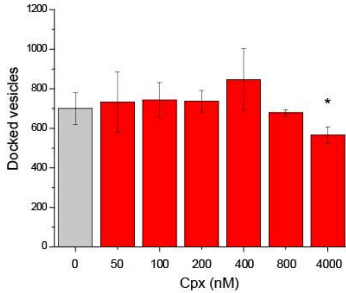
Figure S1. Figure Caption. Vesicle docking is not significantly affected by Cpx. Histogram of the docked v-vesicles harboring both VAMP2 and Syt1 at various concentrations of Cpx. Error bars denote the S.D. of three independent experiments with 5 randomly selected screens shots. Statistical significance was analyzed by the Student's t-test comparing Cpx concentration with no Cpx; *P < 0.05.
