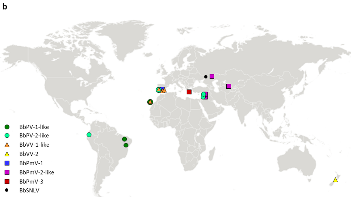
S1 Fig. Population study of dsRNA elements in Beauveria bassiana . (a) Schematic representation of the electrophoretic profiles of dsRNA elements extracted from 17 B. bassiana isolates and their relative sizes. (b) Geographical distribution of mycoviruses found in B. bassiana .
