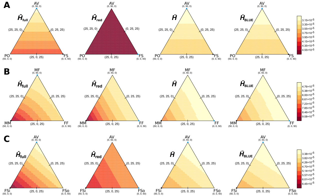
Figure S4: Theoretical mean squared error of \hat{H}_{full} , \hat{H}_{red} , \tilde{H} , and \tilde{H}_{BLUE} for samples fixed at 100 (A) diploid individuals, (B) male and female individuals at an X-linked locus, or (C) diploid individuals wherein some full siblings are inbred with brother-sister parents, across changing sample configurations. The samples were modeled on the D3S2427 locus and contained 50 relative pairs: (A) parent-offspring (PO), second-degree avuncular (AV), and full-sibling (FS), (B) male-male (MM), male-female (MF), and female-female (FF) full-sibling, or (C) inbred full-sibling (FSi), second-degree avuncular (AV), and outbred full-sibling (FSo), such that each individual was related to exactly one other. The vertices of the heat map represent samples composed of only one relative pair type while the space between them corresponds to all possible combinations of relative pair types. Blue and black points indicate the smallest and largest values on the map, respectively. Threshold values for coloration are indicated in the scales to the right of the figure, with smaller values colored lighter.
