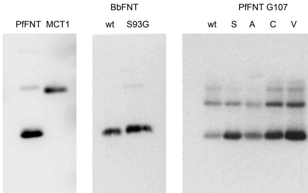
S5 Fig. Expression control by Western blot of PfFNT (38 kDa incl. hemagglutinin epitope and 6xHis tag), rat MCT1 (57 kDa), BbFNT (34 kDa) plus the BbFNT S93G mutant, and the PfFNT G107S/A/C/V mutants. The proteins were detected using a mouse monoclonal anti-hemagglutinin antibody. Each lane was loaded with 30 \mu g of total protein. The appearance of partially SDS-resistant oligomers hints at correct protein folding.
