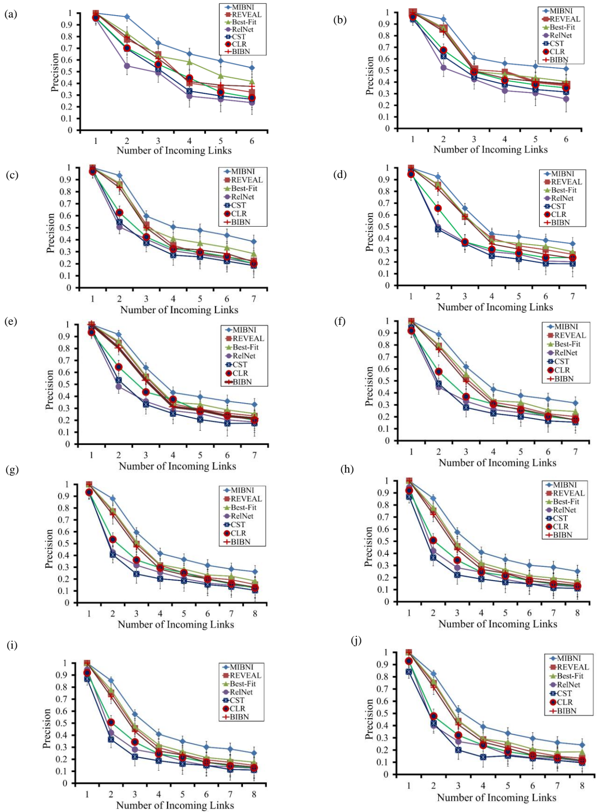
S2 Figure. Comparison of precision between MIBNI and other methods in BA random network groups of different sizes. (a)-(j) Precision results of network groups with |V| = 10, 20, \dots, 100 , respectively. The number of links ( |A| ) was set to 2 \cdot |V| in this work, and 30 BA random networks were examined in each subfigure.
