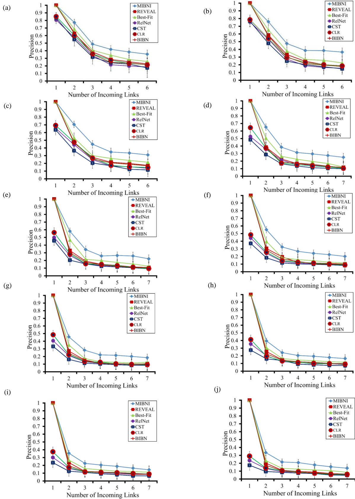
S5 Figure. Comparison of precision between MIBNI and other methods in GNW random network groups of different sizes. (a)-(j) Precision results of network groups with |V| = 10, 20, \dots, 100 , respectively. In each subfigure, 30 GNW random networks were examined.
