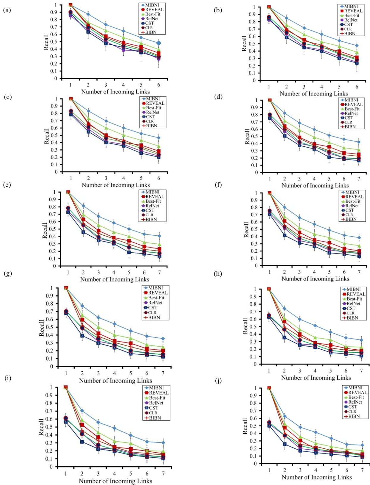
S6 Figure. Comparison of recall between MIBNI and other methods in GNW random network groups of different sizes. (a)-(j) Recall results of network groups with |V| = 10, 20, \dots, 100 , respectively. In each subfigure, 30 GNW random networks were examined.
