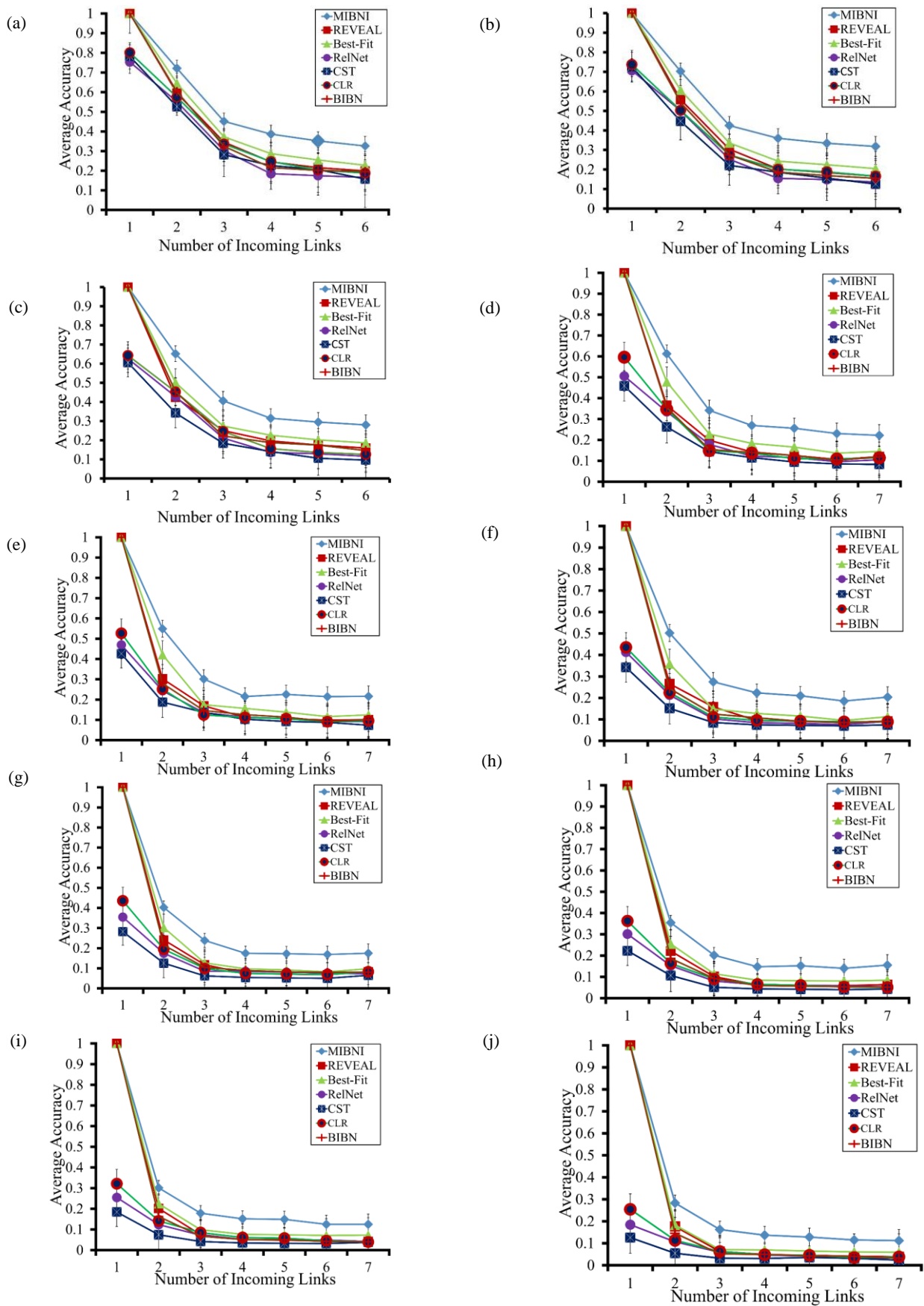
S7 Figure. Comparison of structural accuracy between MIBNI and other methods in GNW random network groups of different sizes. (a)-(j) Recall results of network groups with |V| = 10, 20, \dots, 100 , respectively. In each subfigure, 30 GNW random networks were examined.
