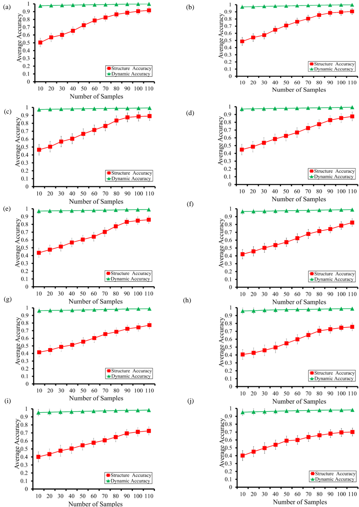
S9 Figure. Changes of structural and dynamics accuracy of MIBNI in BA random network groups against the number of samples. (a)-(j) Structural accuracy results of network groups with |V| = 10, 20, \dots, 100 , respectively. The number of links ( |A| ) was set to 2 \cdot |V| in this work, and 30 BA random networks were examined in each subfigure. The maximum time step (i.e., the number of samples) in gene expression datasets varies from 10 to 110 by 10.
