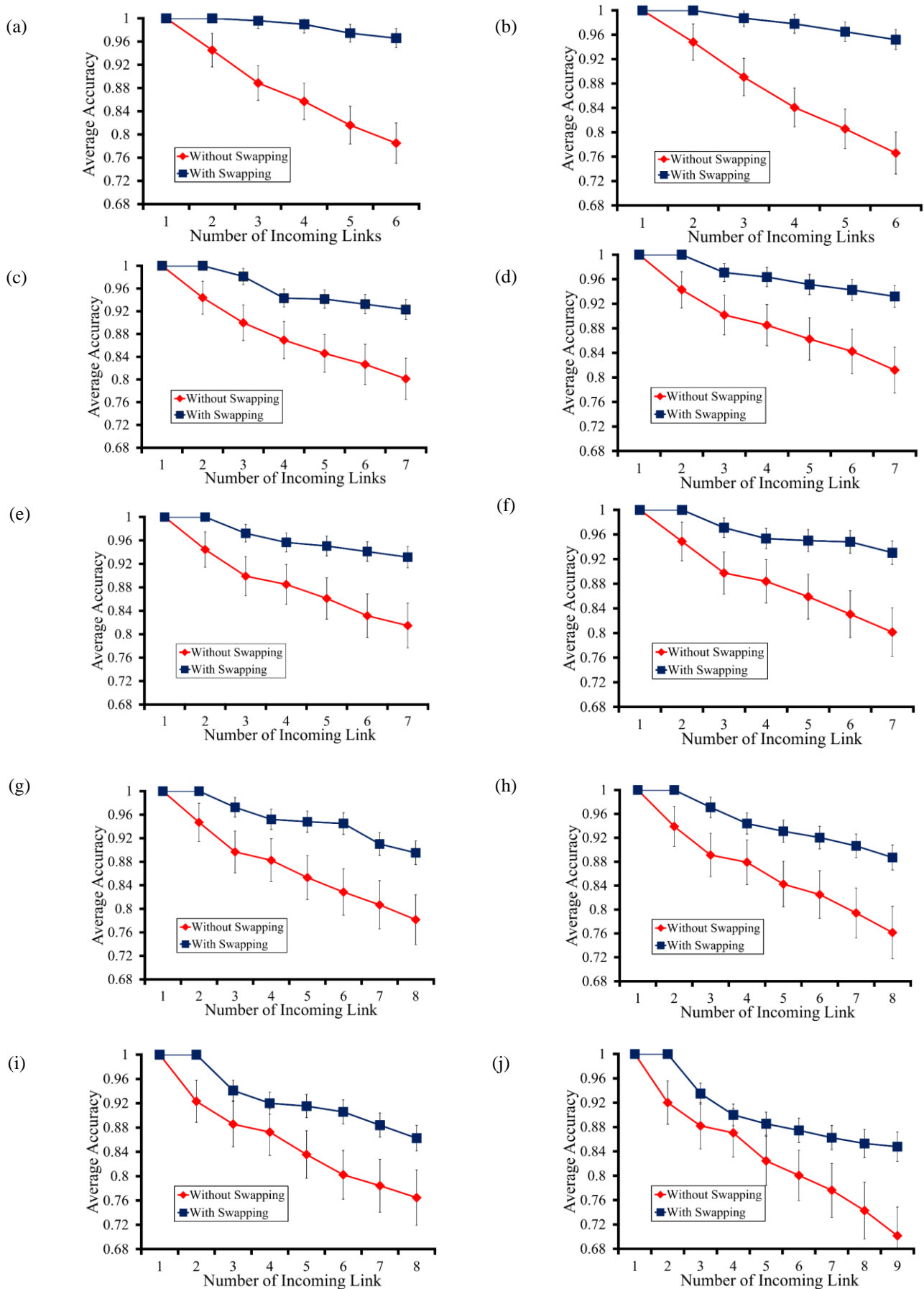
S10 Figure. Performance improvement by SWAP subroutine in BA random network groups of different sizes. (a)-(j) Results of network groups with |V| = 10, 20, \dots, 100 , respectively. The number of links ( |A| ) was set to 2 \cdot |V| , and 30 BA random networks were examined in each subfigure. The Y-axis values show changes in the average dynamic accuracies versus the number of incoming links.
