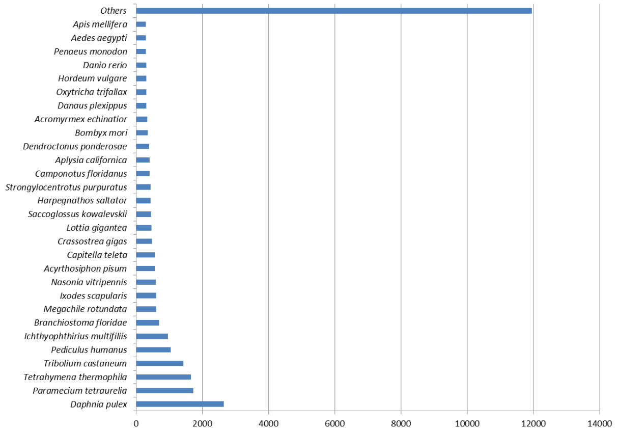
Figure S1: Top hit species distribution chart. X-axis represents the number of blast matches while Y-axis shows the name of different species.
