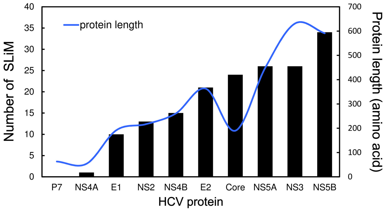
S10 Fig. The number of conserved (in \geq 70\% sequences) SLiMs found in HCV component proteins and protein length.
