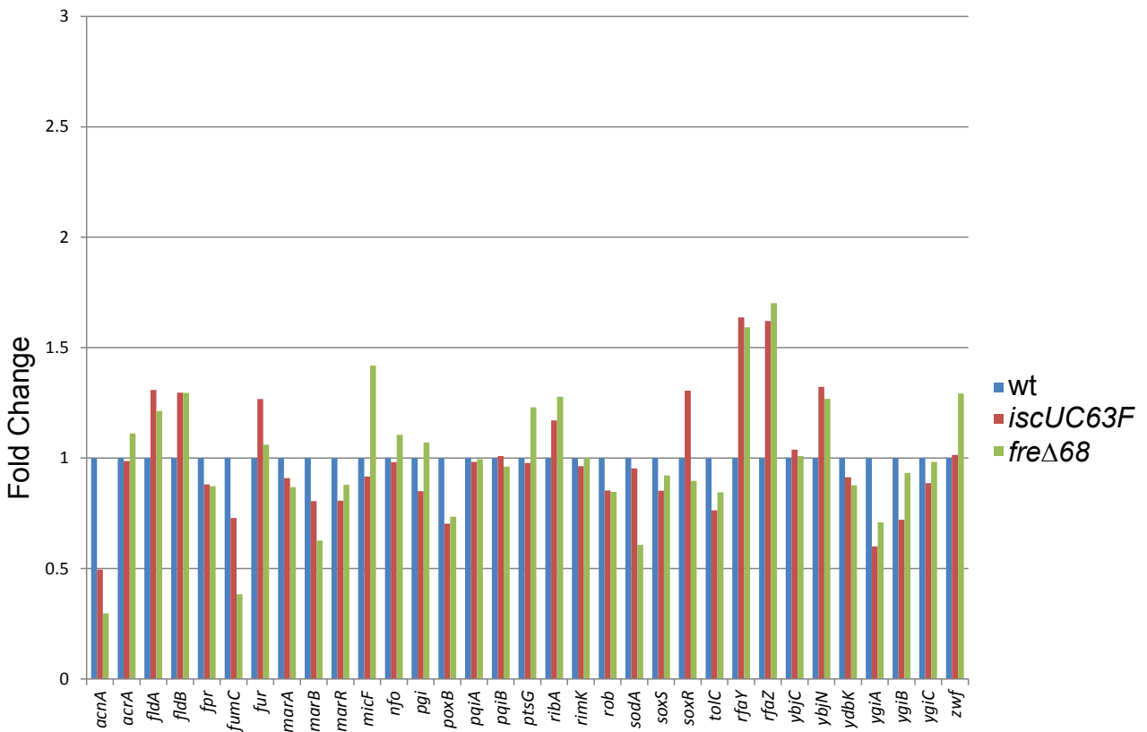
S5 Fig. The OxyR and SoxRS regulons in iscU and fre mutants. The expression level of selected OxyR and SoxRS controlled genes relative to wild-type extracted from the microarray experiment.
